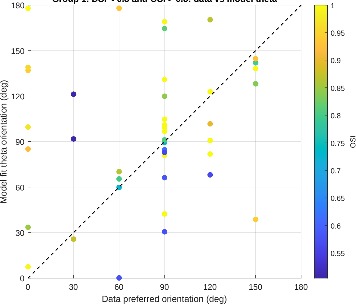
Group 1: DSI < 0.3 and OSI > 0.5: data vs model theta
