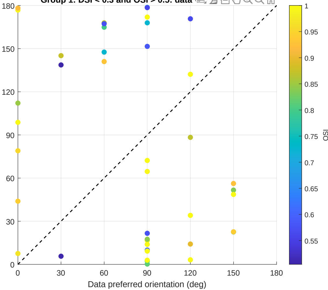
Group 1: DSI < 0.3 and OSI > 0.5: data
