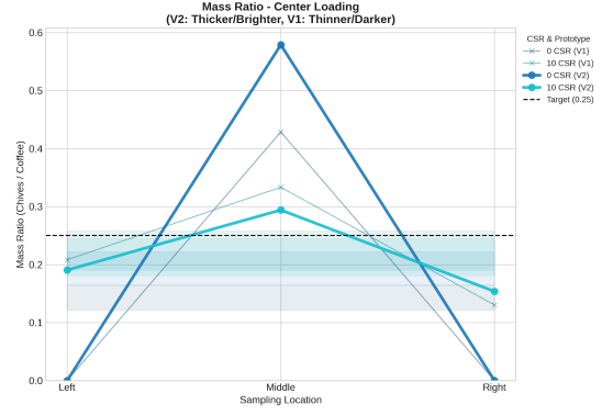
Figure 3: Paddle geometry comparison when central loaded
