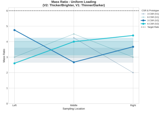
Figure 2: Paddle geometry comparison when uniformly loaded
