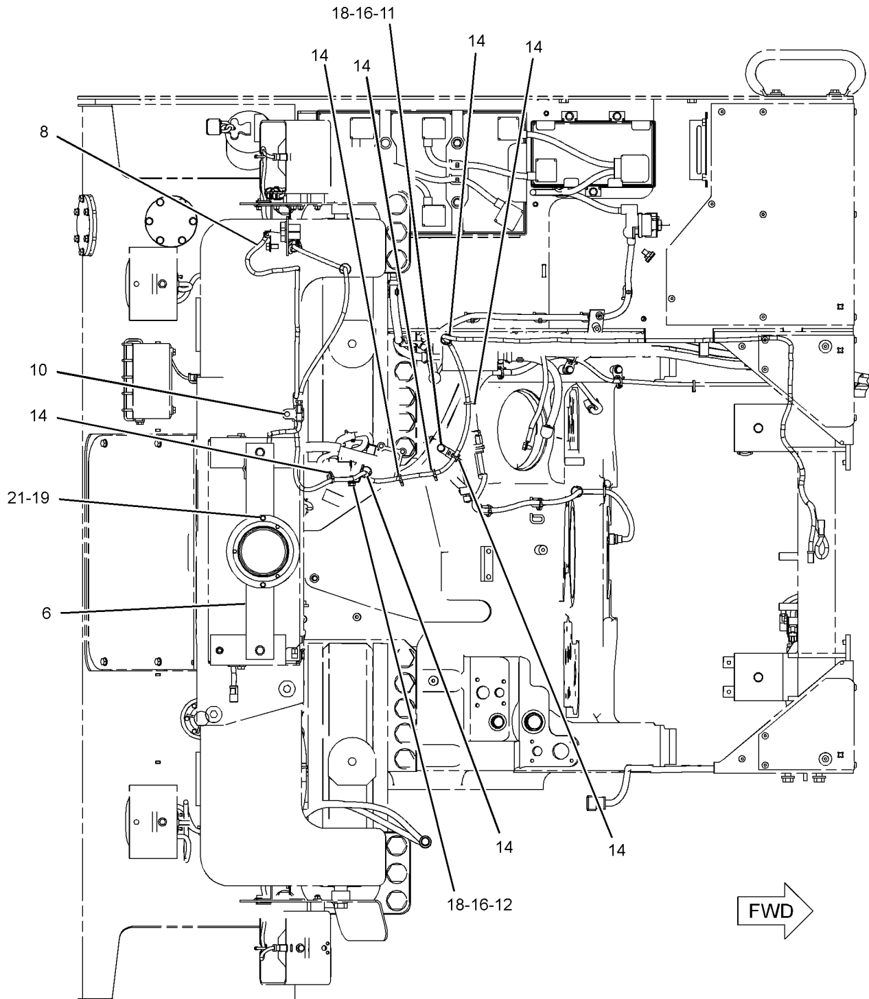
TOP VIEW (PLATFORM AND CABIN REMOVED)
