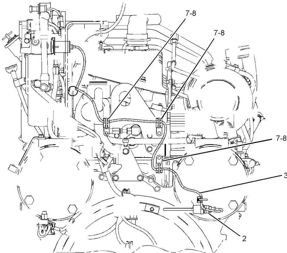
REAR VIEW
