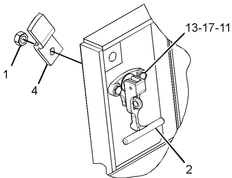
VIEW OF AREA A (EXPLODED)
