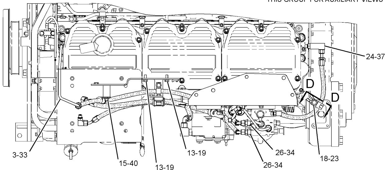
TOP VIEW OF ENGINE
