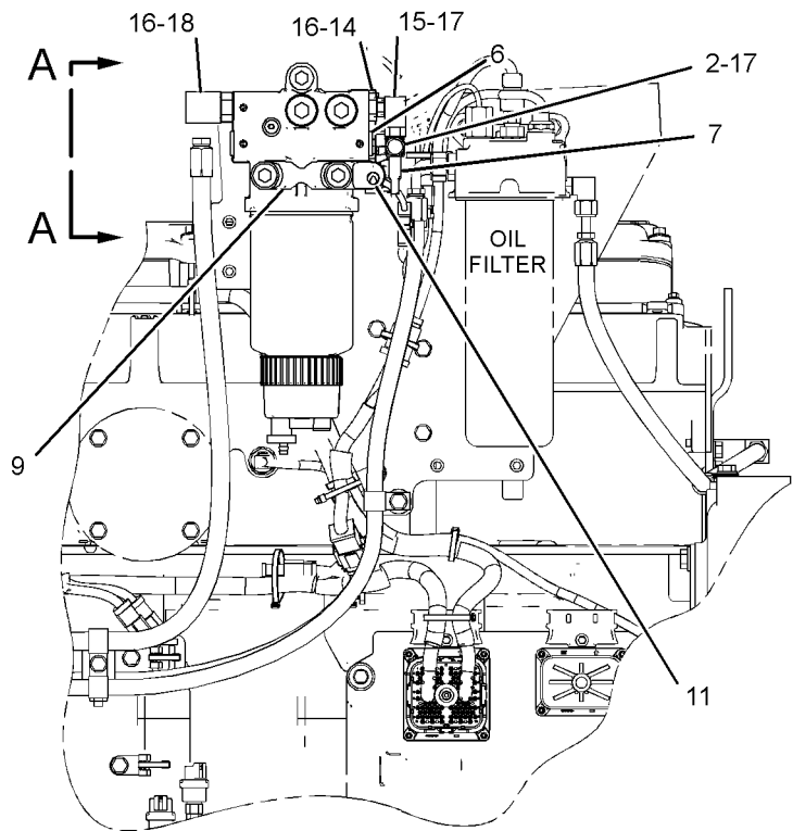
LEFT SIDE VIEW OF ENGINE
