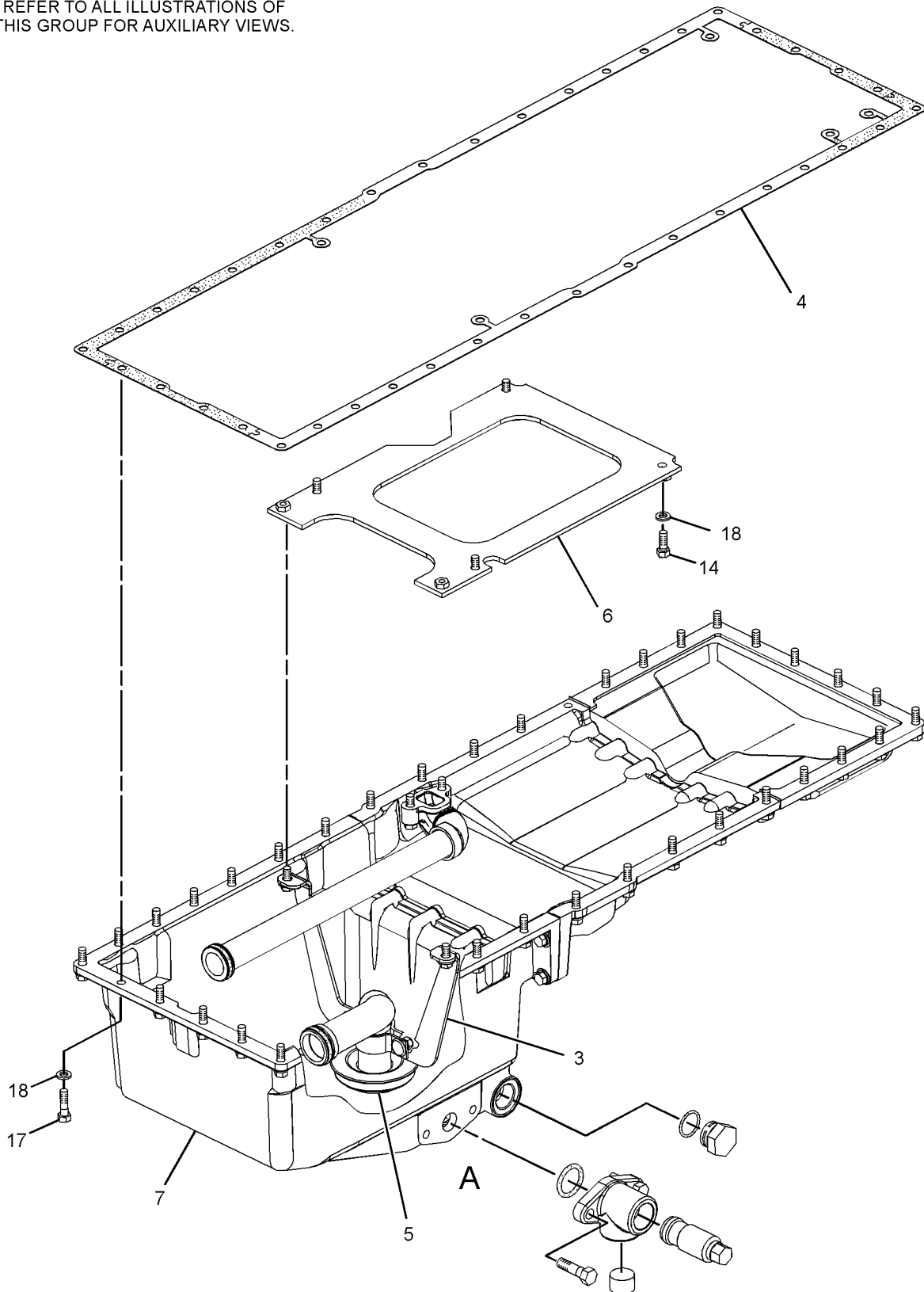
GRAPHIC #1
