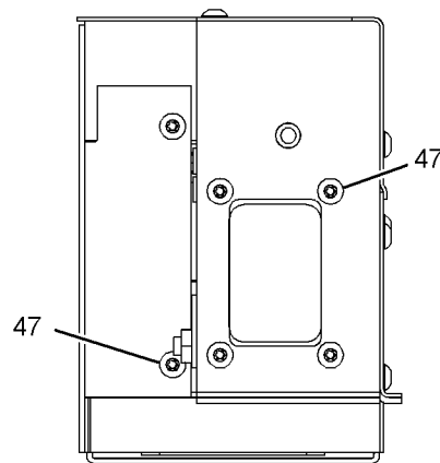
VIEW F-F
