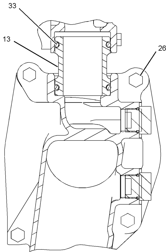
SECTION B-B
