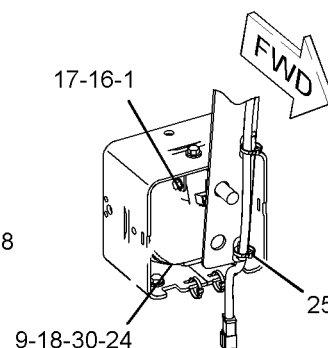
VIEW OF SECTION C-C
