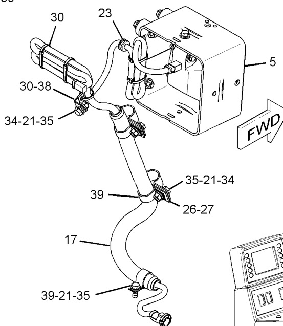
VIEW OF AREA B
