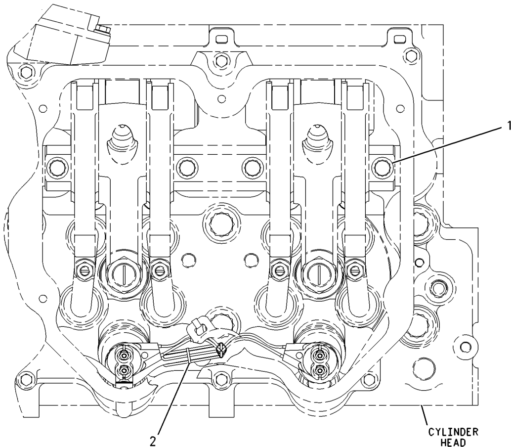
TOP VIEW
