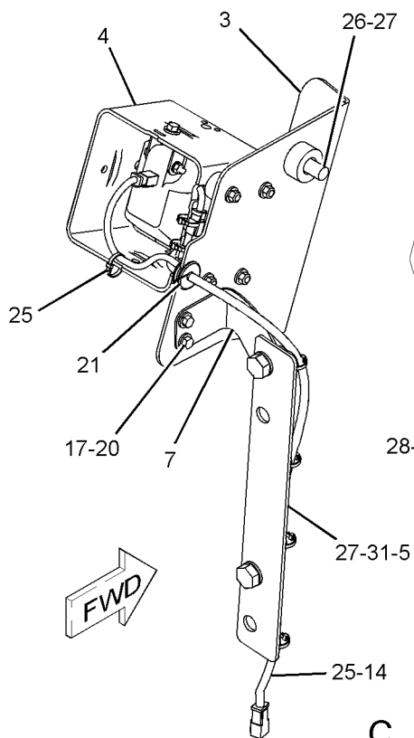
REAR VIEW OF ROPS
