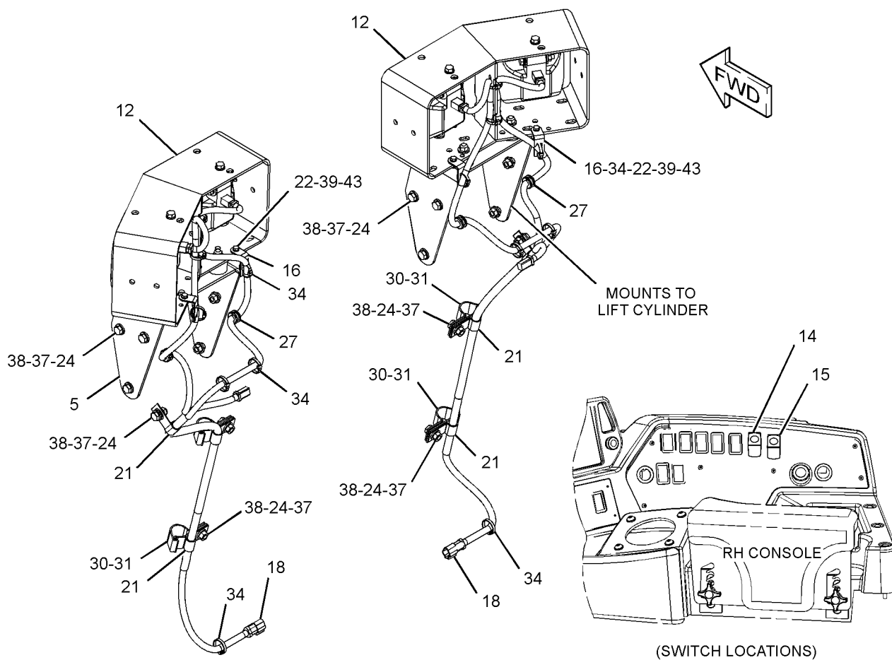
GRAPHIC #1
