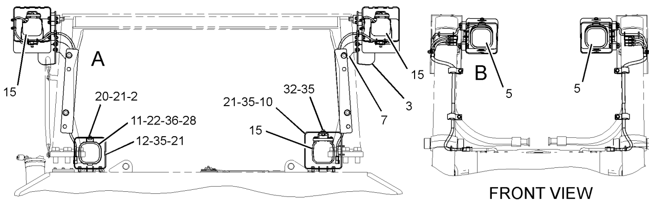
REAR VIEW OF ROPS
