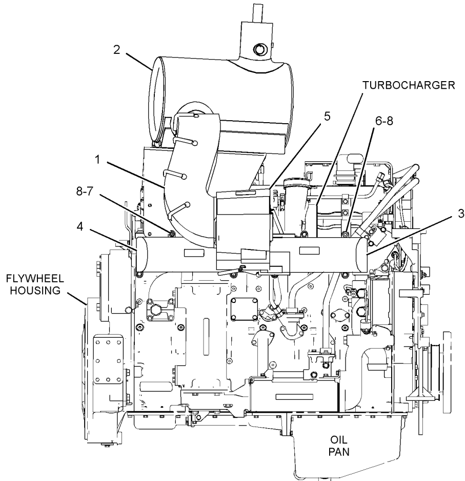
RIGHT SIDE VIEW OF ENGINE <END>
