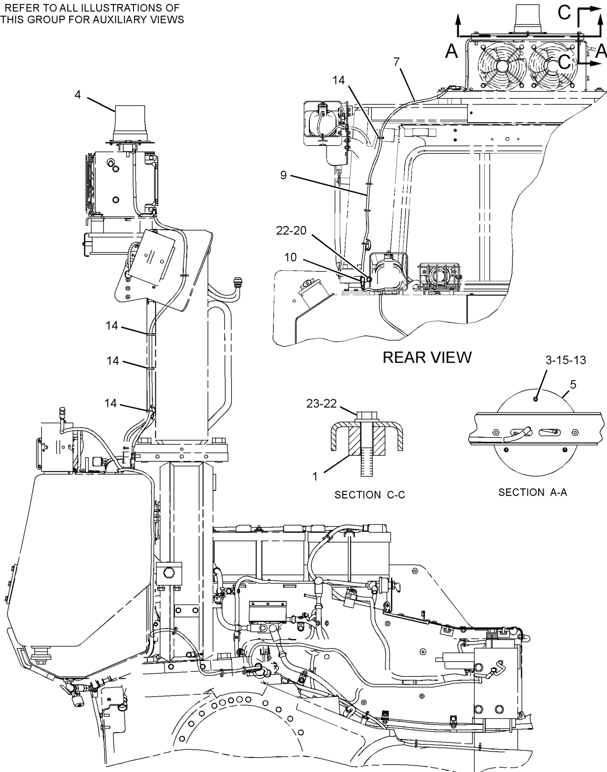
RIGHT SIDE VIEW (PLATFORM AND CABIN REMOVED)
