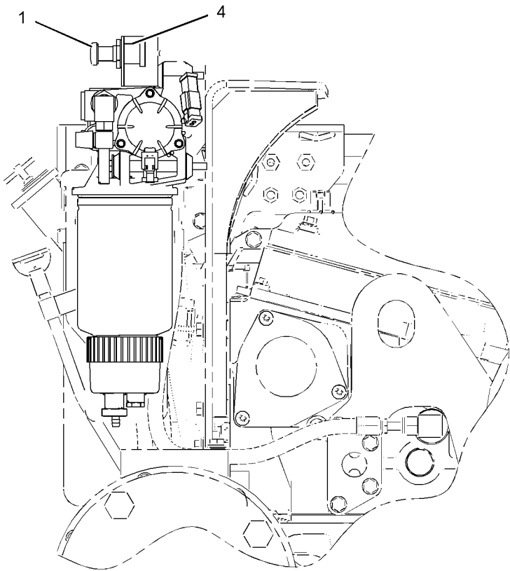
REAR VIEW
