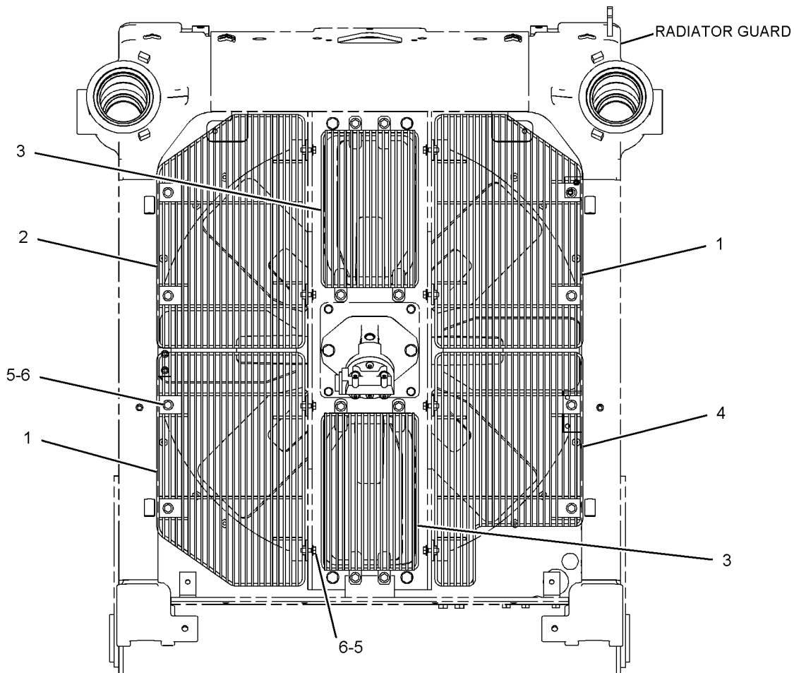
REAR VIEW <END>
