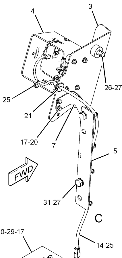
REAR VIEW OF ROPS
