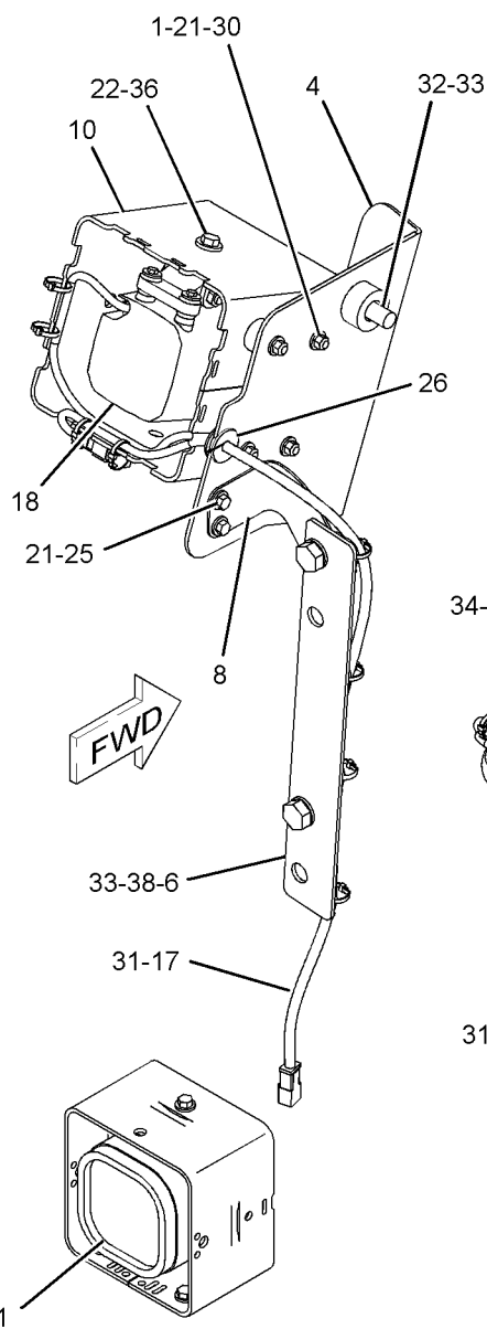
VIEW OF AREA A
