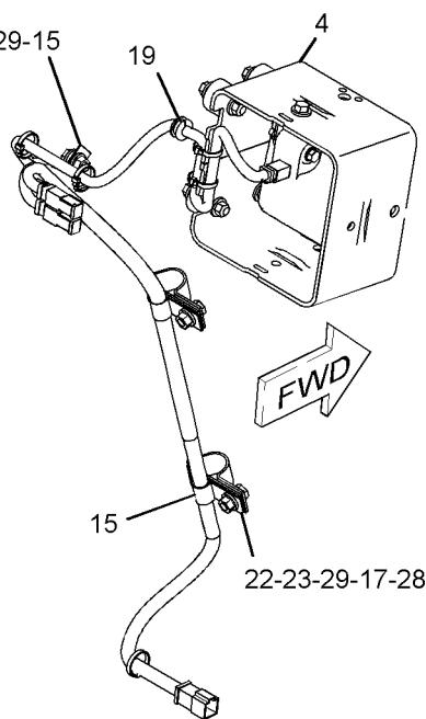
VIEW OF AREA B
