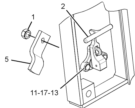
VIEW OF AREA B (EXPLODED)
