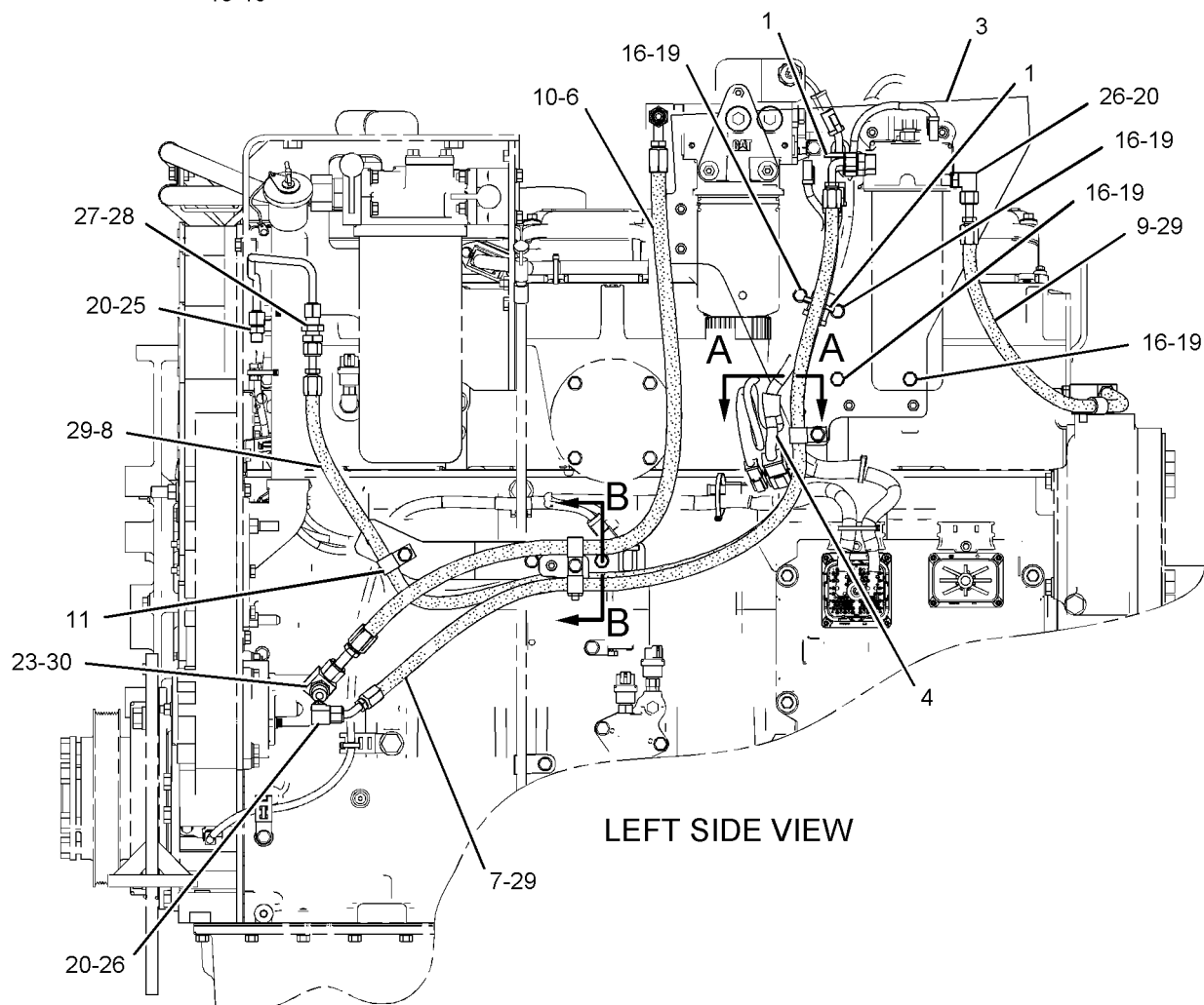
GRAPHIC #1
