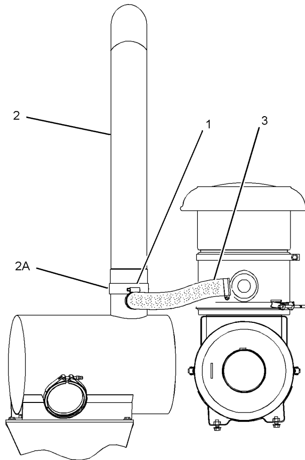
RIGHT SIDE VIEW <END>
