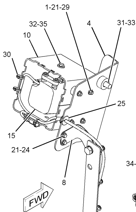
REAR VIEW OF ROPS
