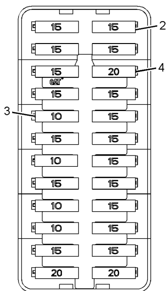
(VIEW OF FUSE LOCATIONS)
