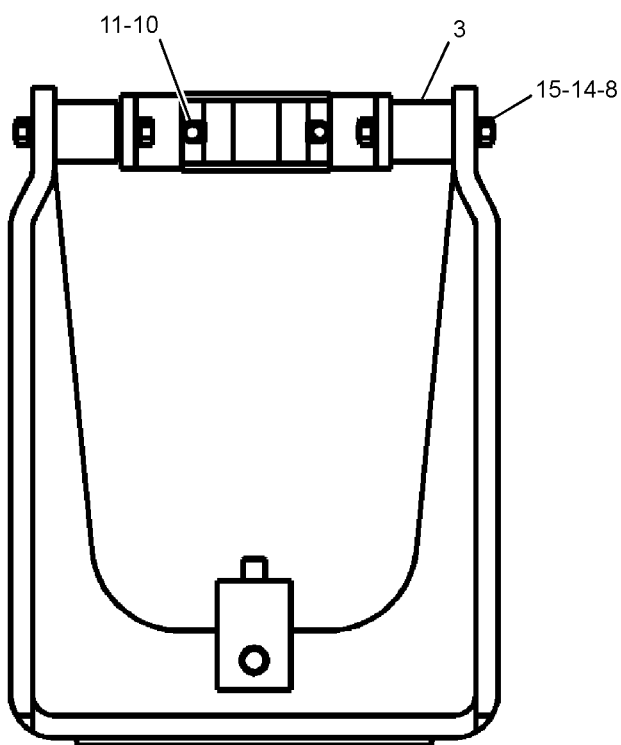
VIEW B-B
