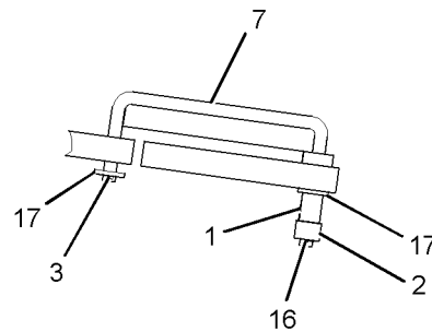
VIEW C-C
