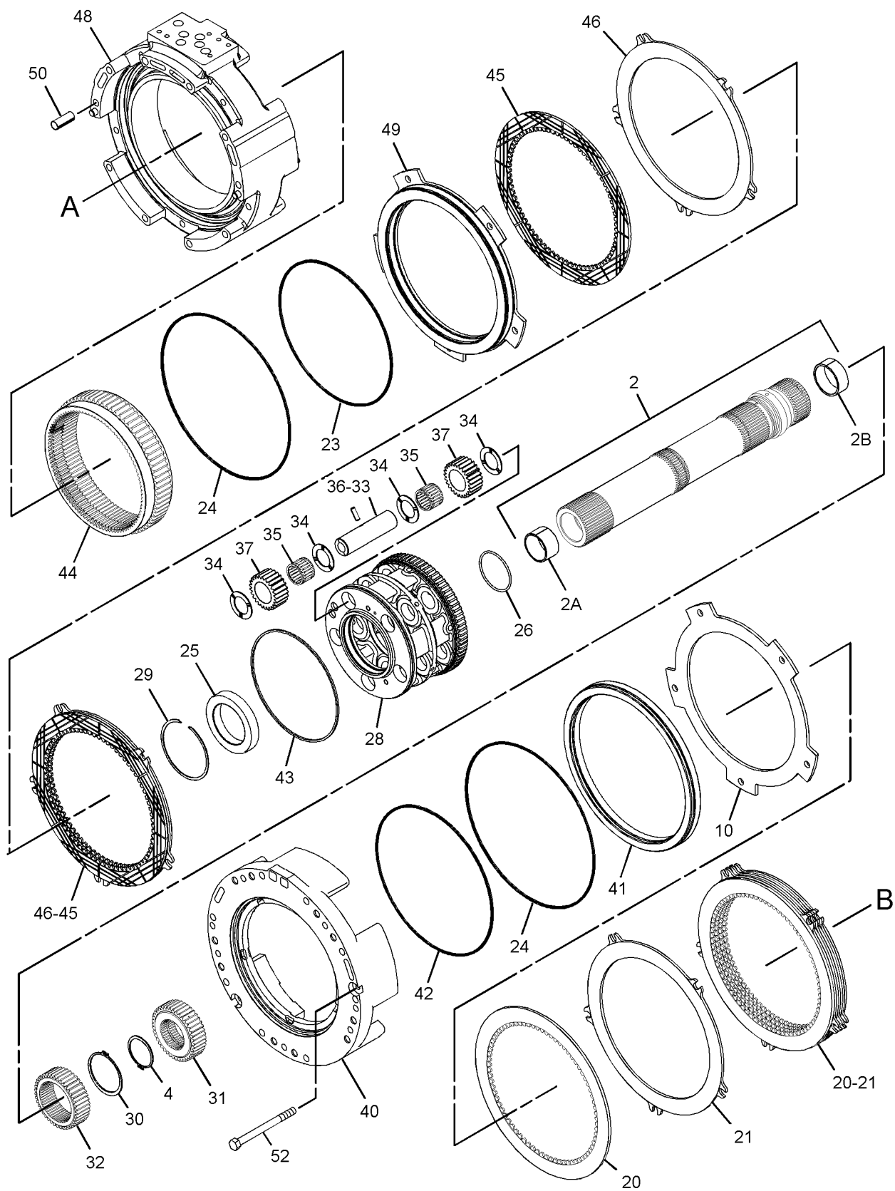
GRAPHIC #2
