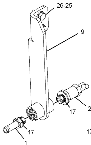
VIEW OF AREA D (EXPLODED)
