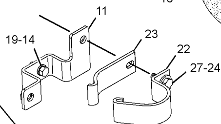
VIEW OF AREA (EXPLODED)
