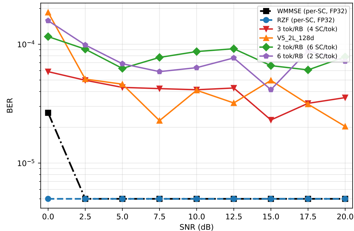
(b) Bit Error Rate (Monte Carlo accumulation)
