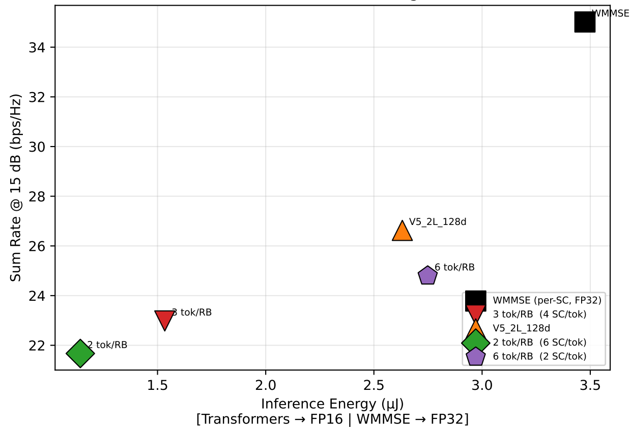
(c) Energy-Performance Pareto (RZF excluded — see Fig. 2)
