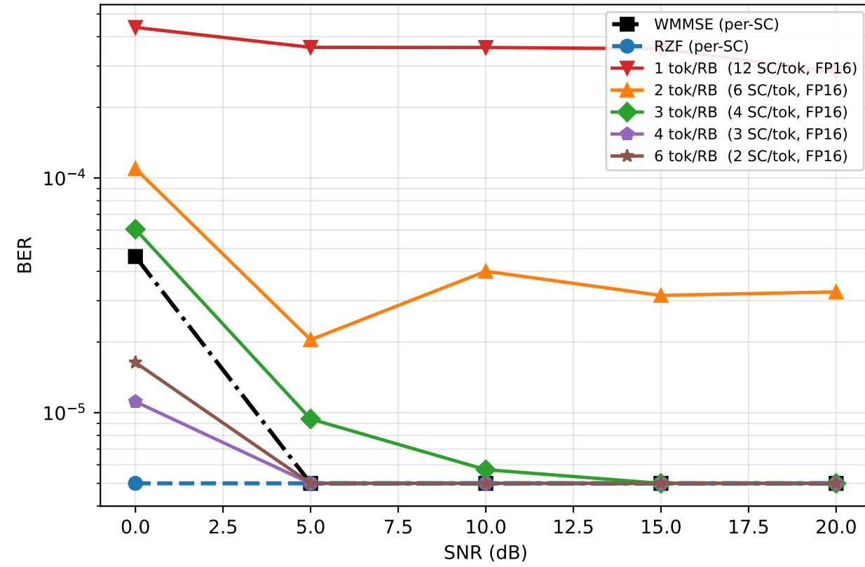
(b) Bit Error Rate (Monte Carlo)
