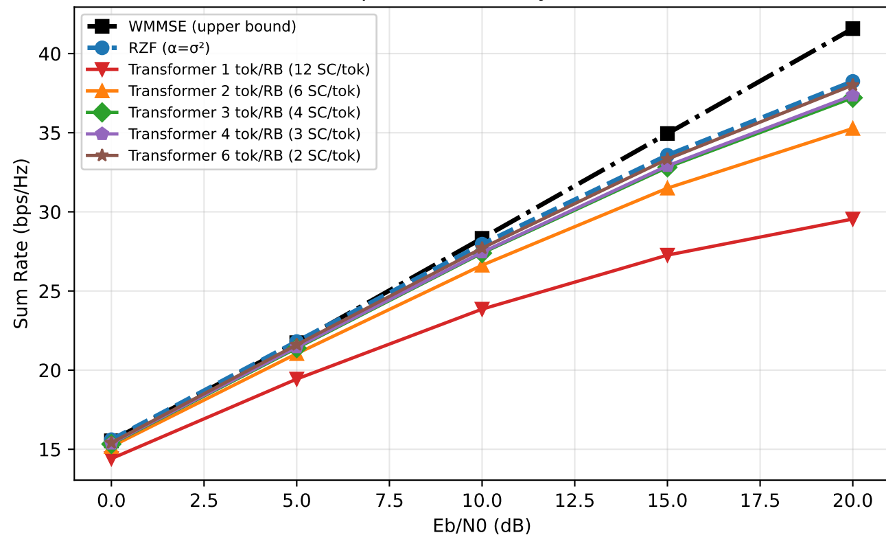
(a) Spectral Efficiency vs Eb/N0
