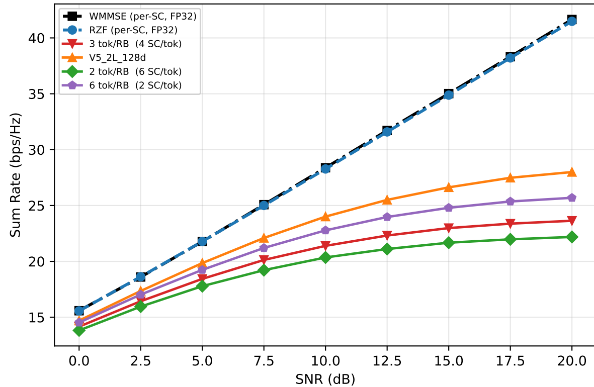
(a) Full Comparison — Transformer vs RZF Grouping
