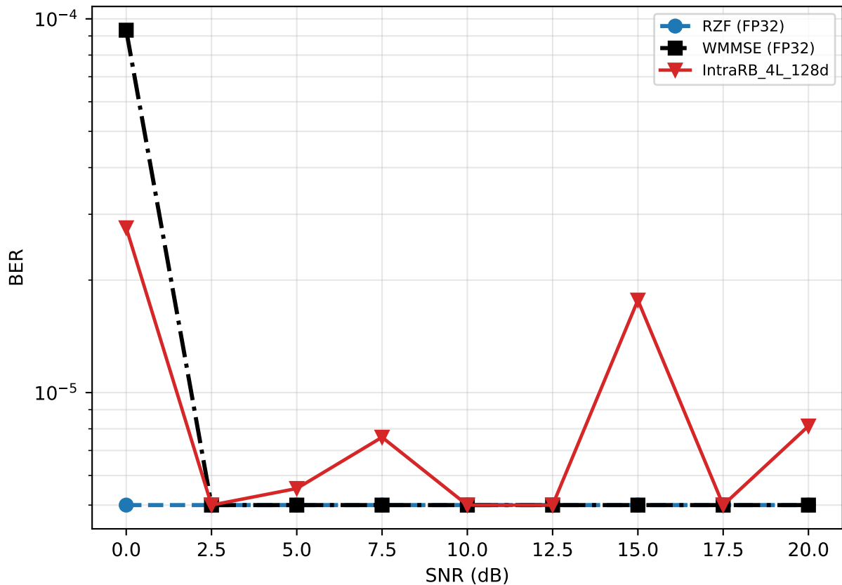
(b) BER Monte Carlo
