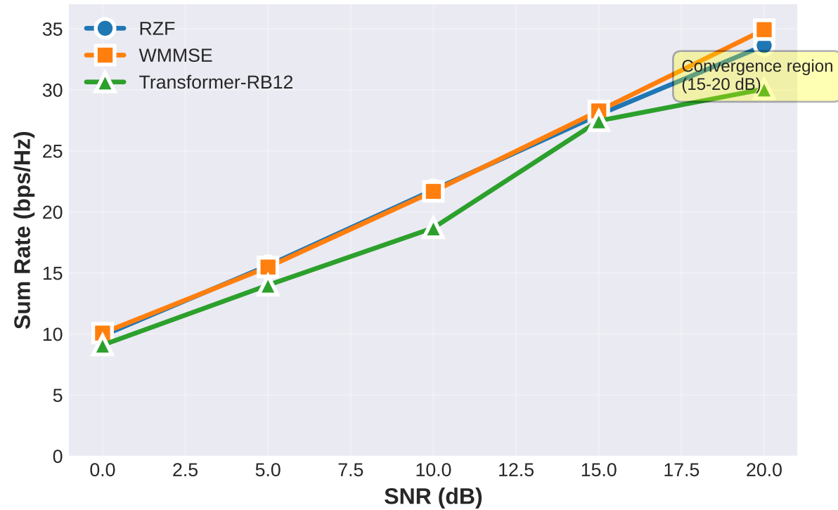
(a) Spectral Efficiency vs SNR
