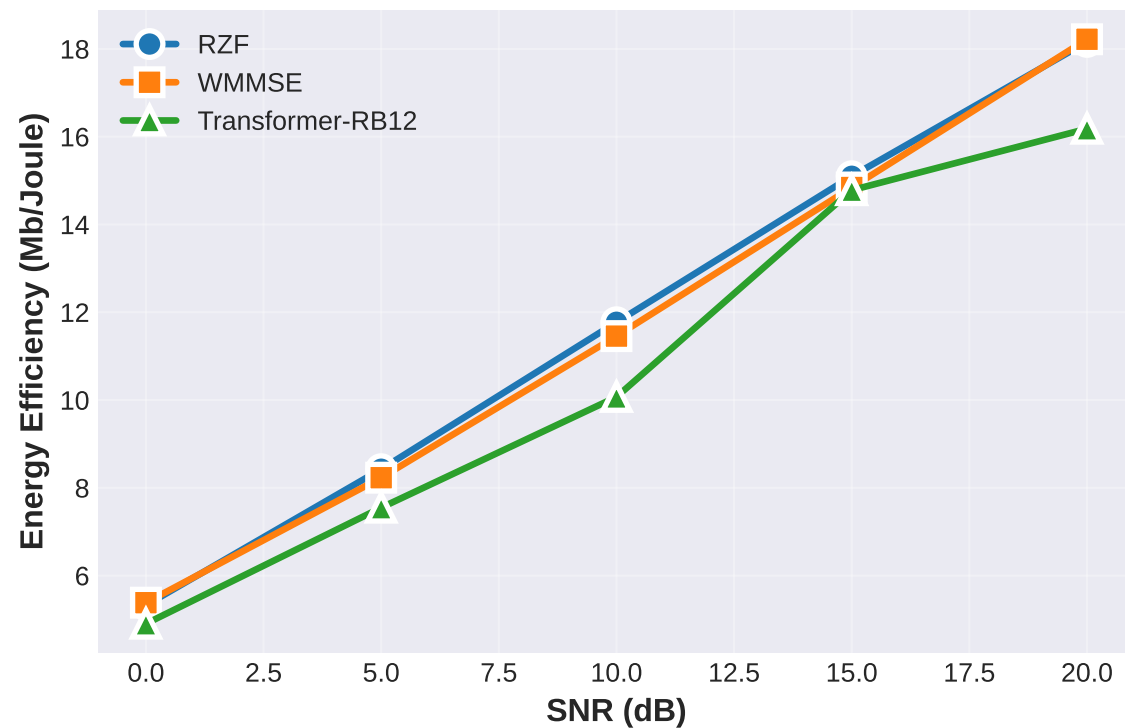
(c) Energy Efficiency (KPI #1)
