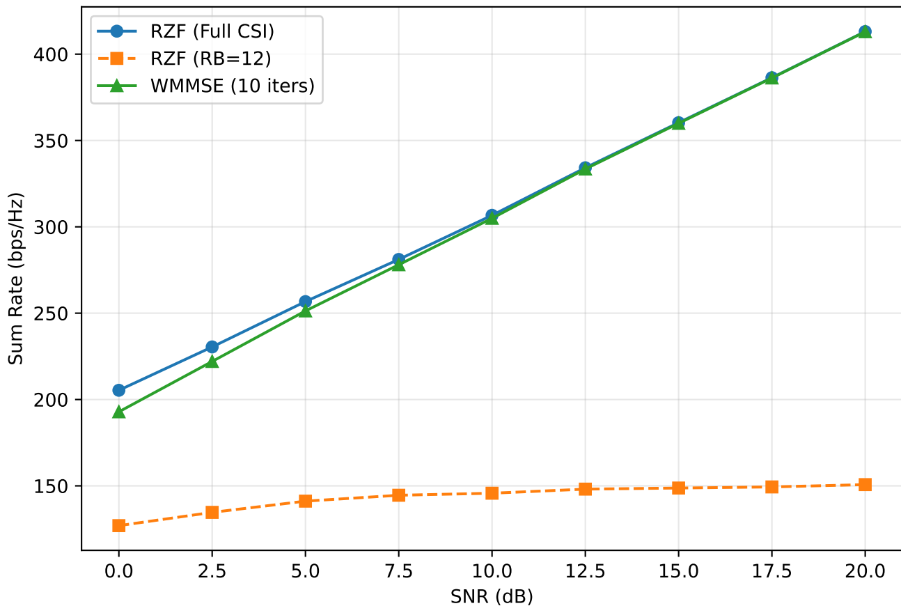
M64K32 (CPU-verified): RZF vs WMMSE
