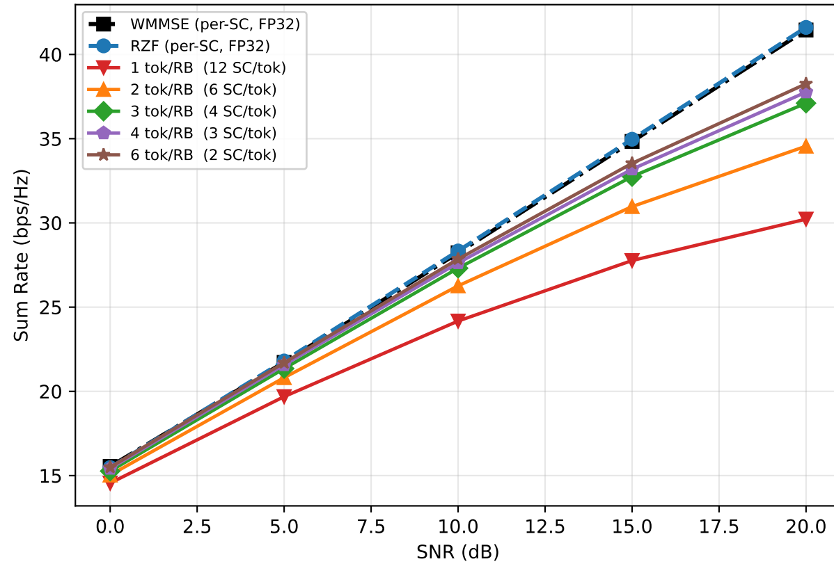
(a) Spectral Efficiency
