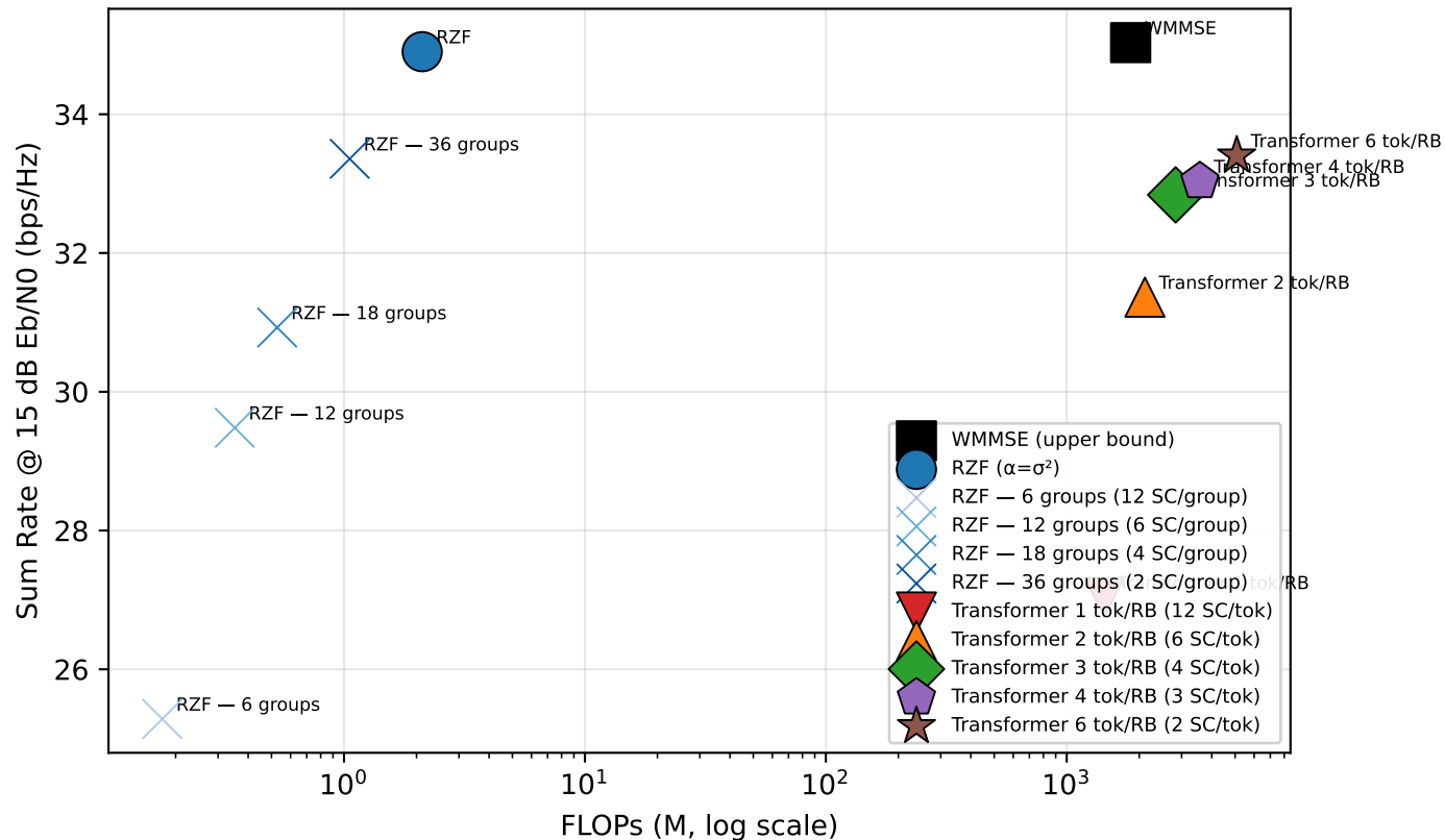
(b) Complexity-Performance Pareto
