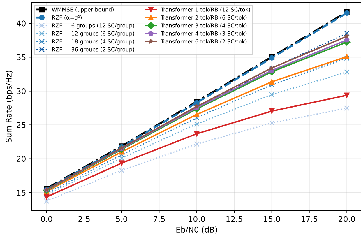
(a) Transformer vs RZF Grouping
