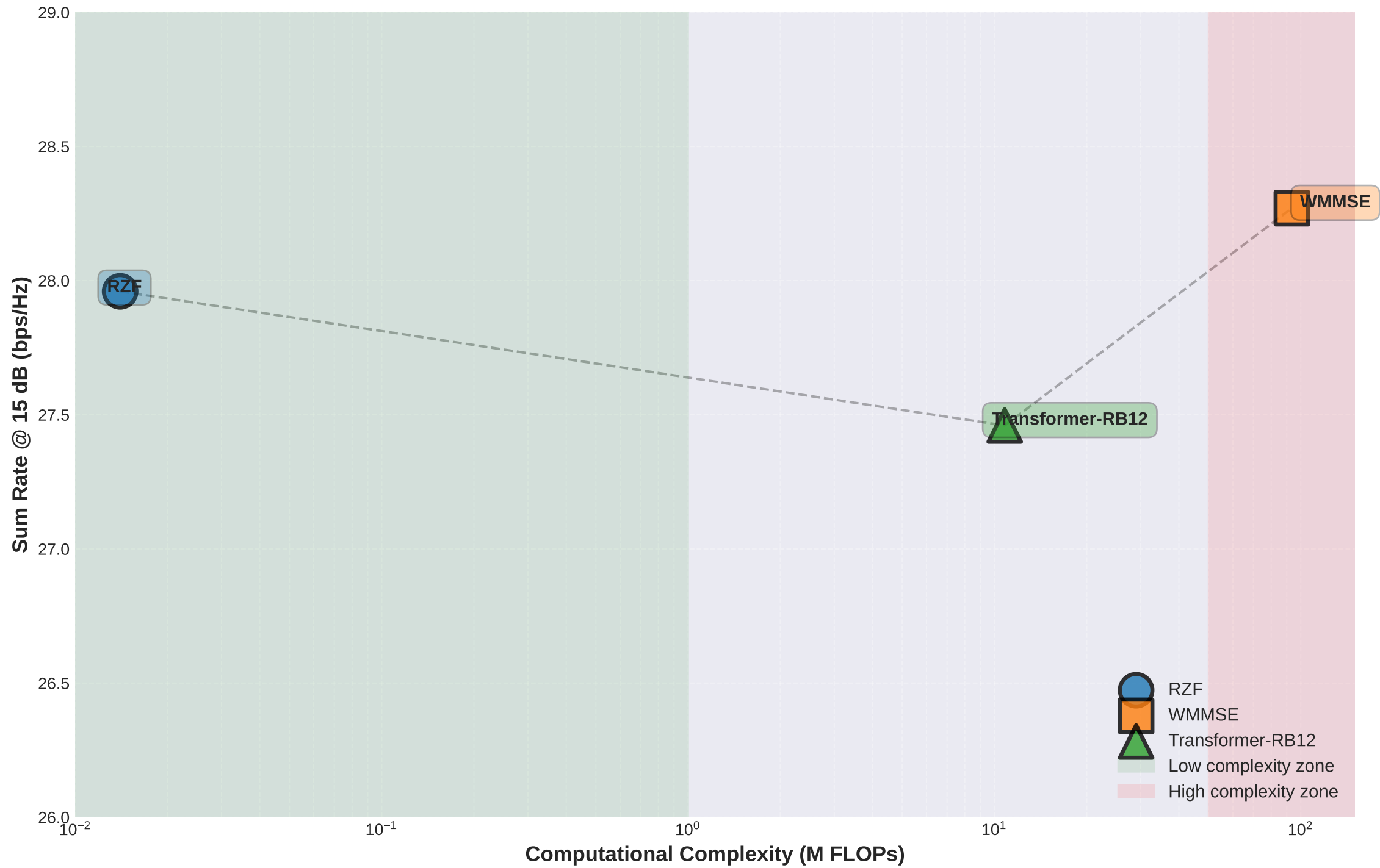
Complexity-Performance Trade-off @ 15 dB SNR
