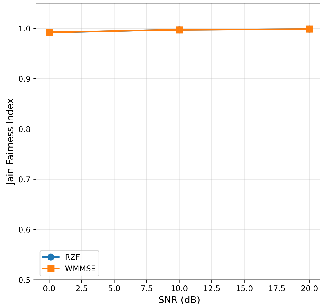
User Fairness vs SNR
