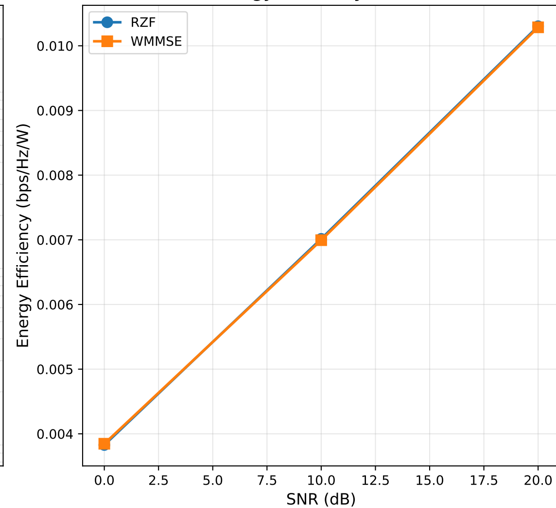
Energy Efficiency Improvement
