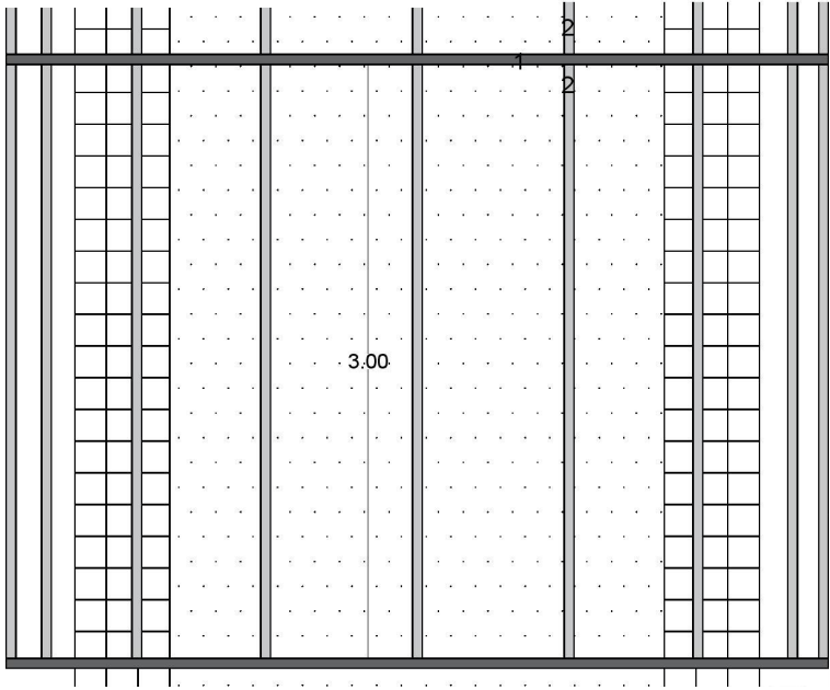
Pergola Topview
