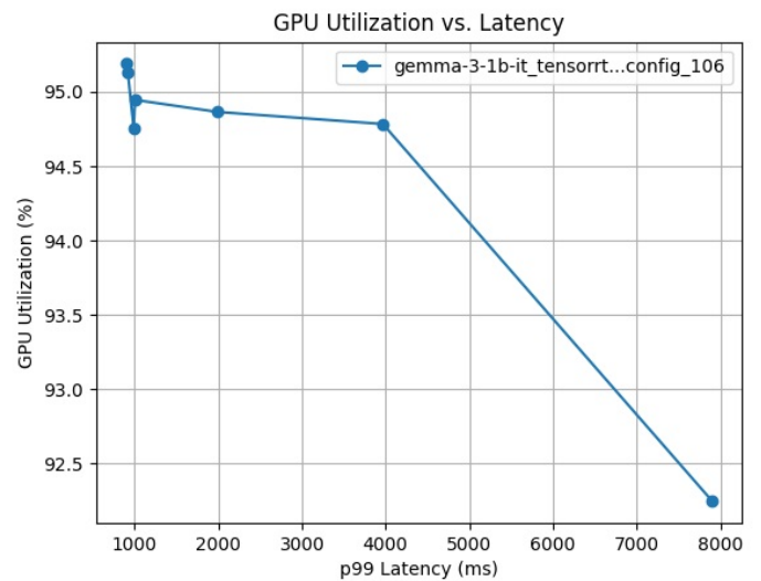
GPU Utilization vs. Latency curves for config gemma-3-1b-it_tensorrt_llm_bls_config_106
