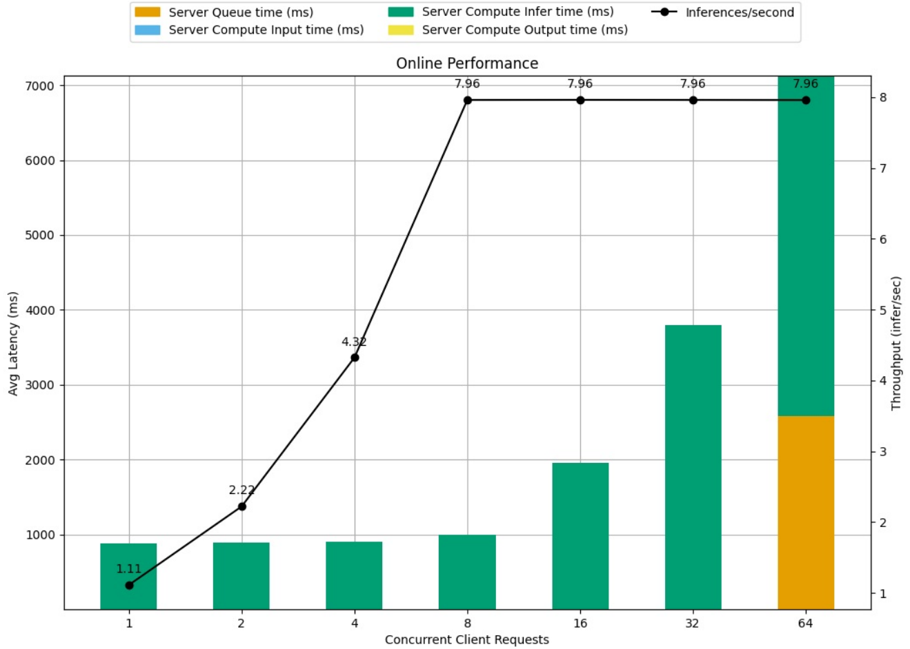
Latency Breakdown for Online Performance of gemma-3-1b-it_tensorrt_llm_bls_config_106
