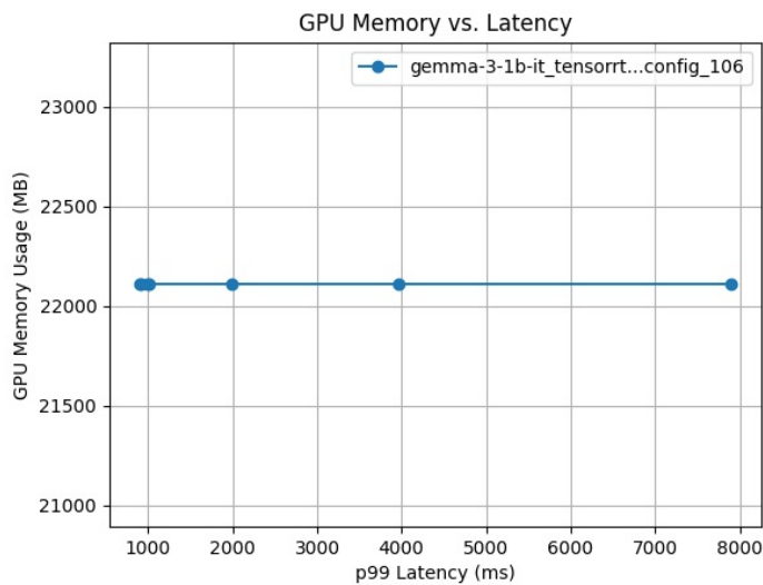
GPU Memory vs. Latency curves for config gemma-3-1b-it_tensorrt_llm_bls_config_106
