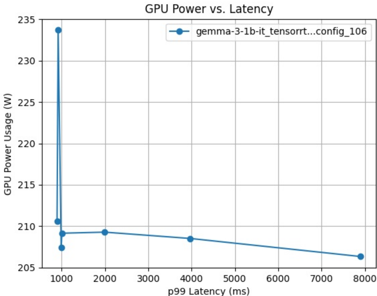
GPU Power vs. Latency curves for config gemma-3-1b-it_tensorrt_llm_bls_config_106
