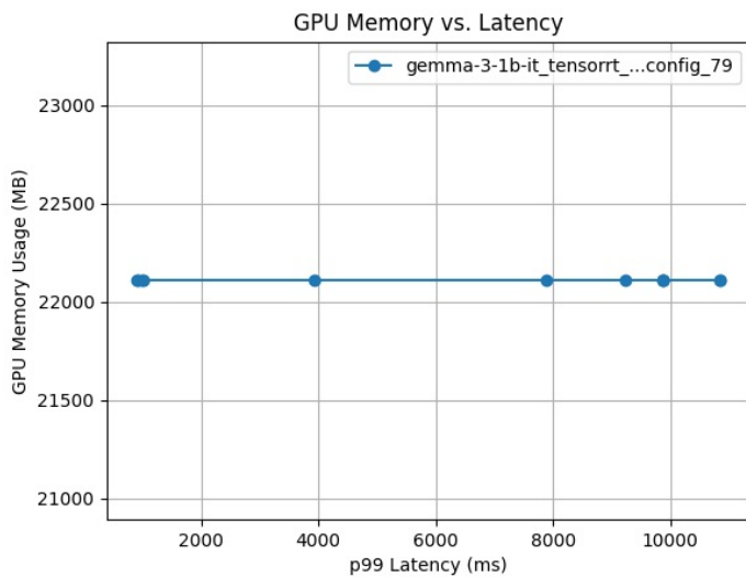
GPU Memory vs. Latency curves for config gemma-3-1b-it_tensorrt_llm_bls_config_79
