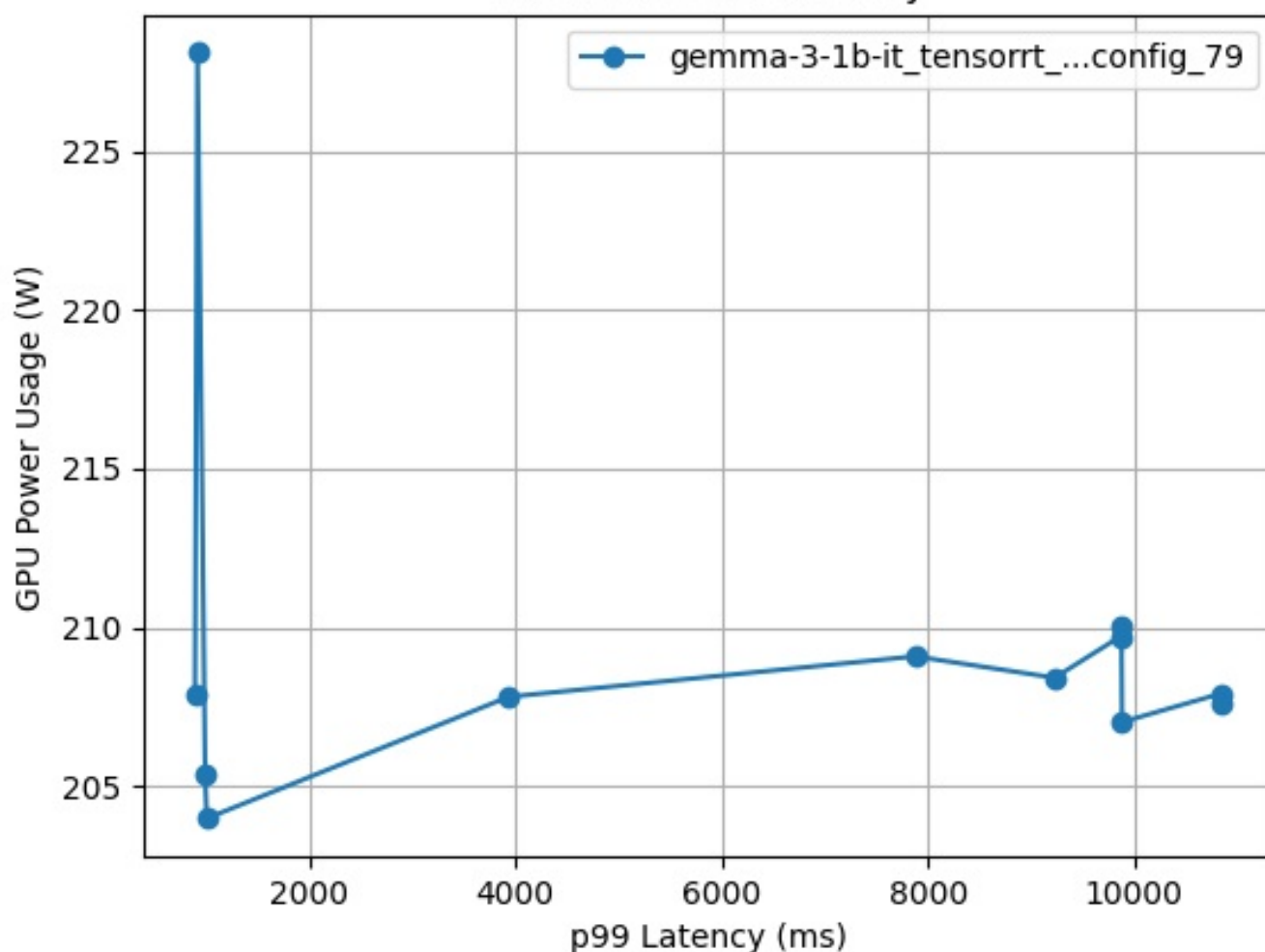
GPU Power vs. Latency curves for config gemma-3-1b-it_tensorrt_llm_bls_config_79
