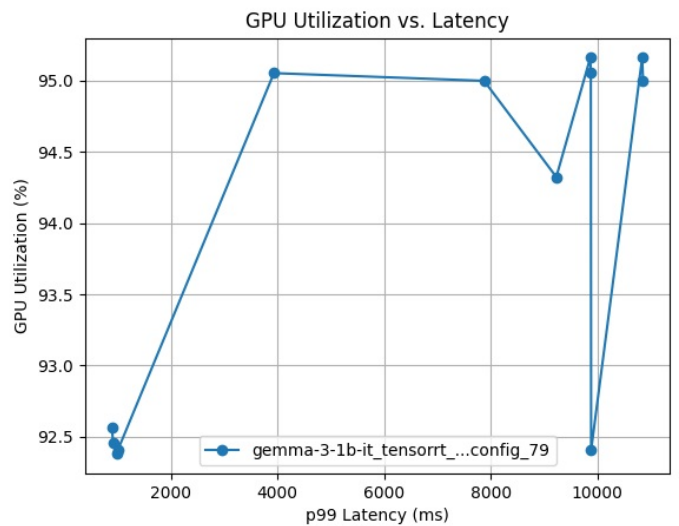
GPU Utilization vs. Latency curves for config gemma-3-1b-it_tensorrt_llm_bls_config_79
