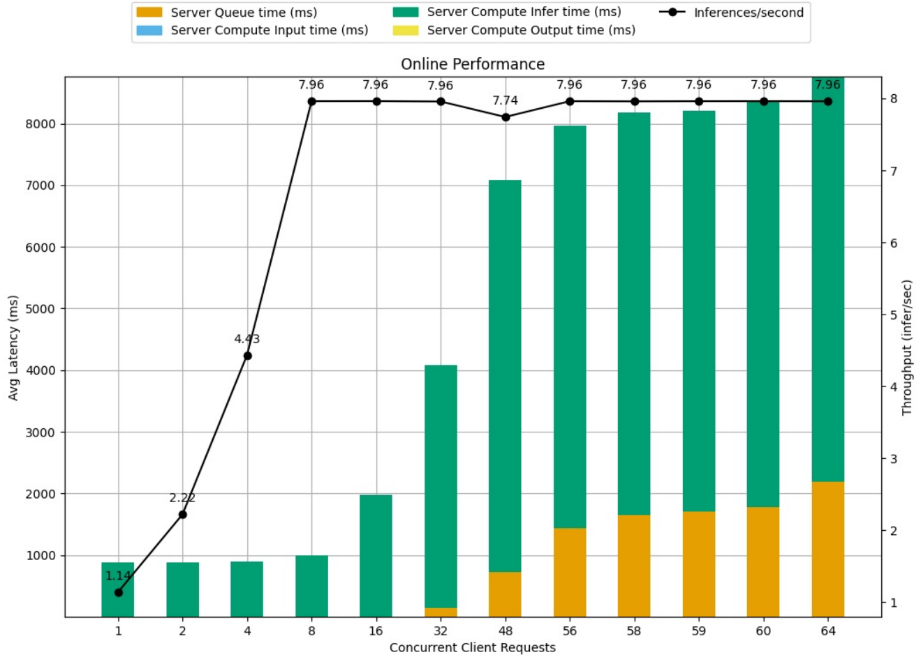
Latency Breakdown for Online Performance of gemma-3-1b-it_tensorrt_llm_bls_config_79
