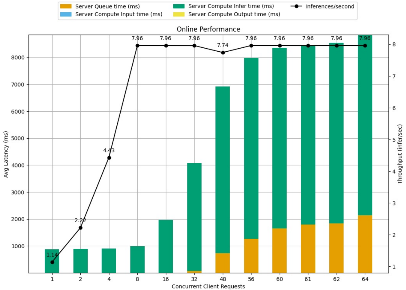
Latency Breakdown for Online Performance of gemma-3-1b-it_tensorrt_llm_bls_config_82
