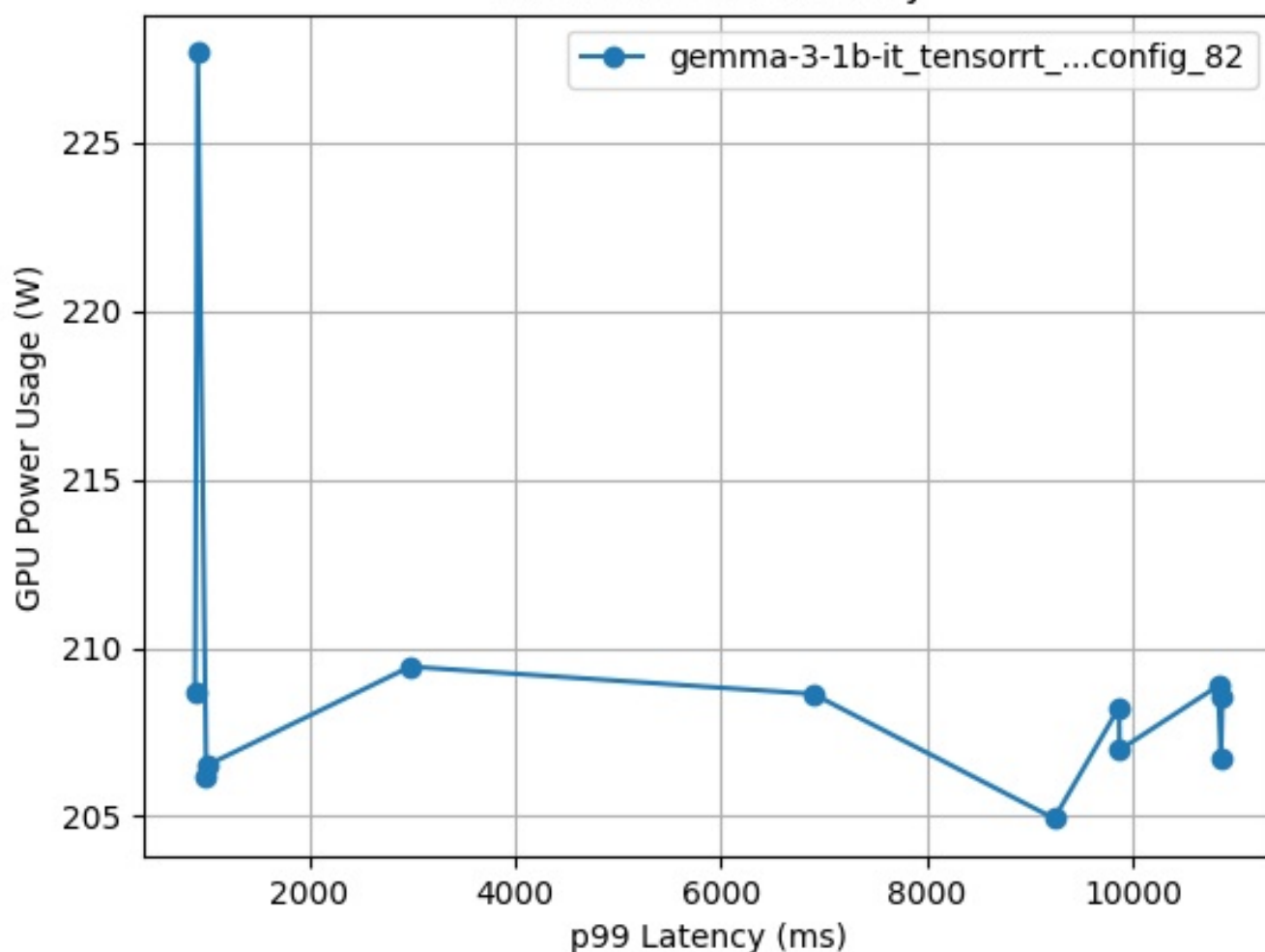
GPU Power vs. Latency curves for config gemma-3-1b-it_tensorrt_llm_bls_config_82
