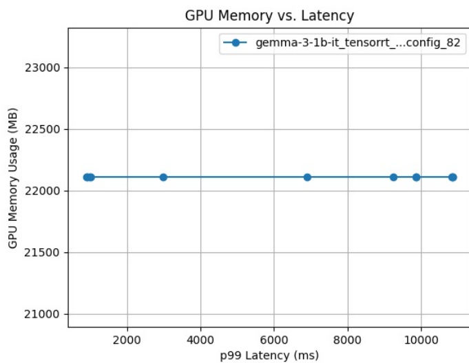
GPU Memory vs. Latency curves for config gemma-3-1b-it_tensorrt_llm_bls_config_82
