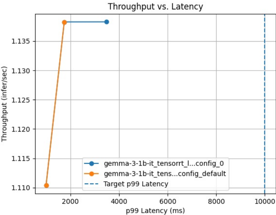
Throughput vs. Latency curves for 2 best configurations.
