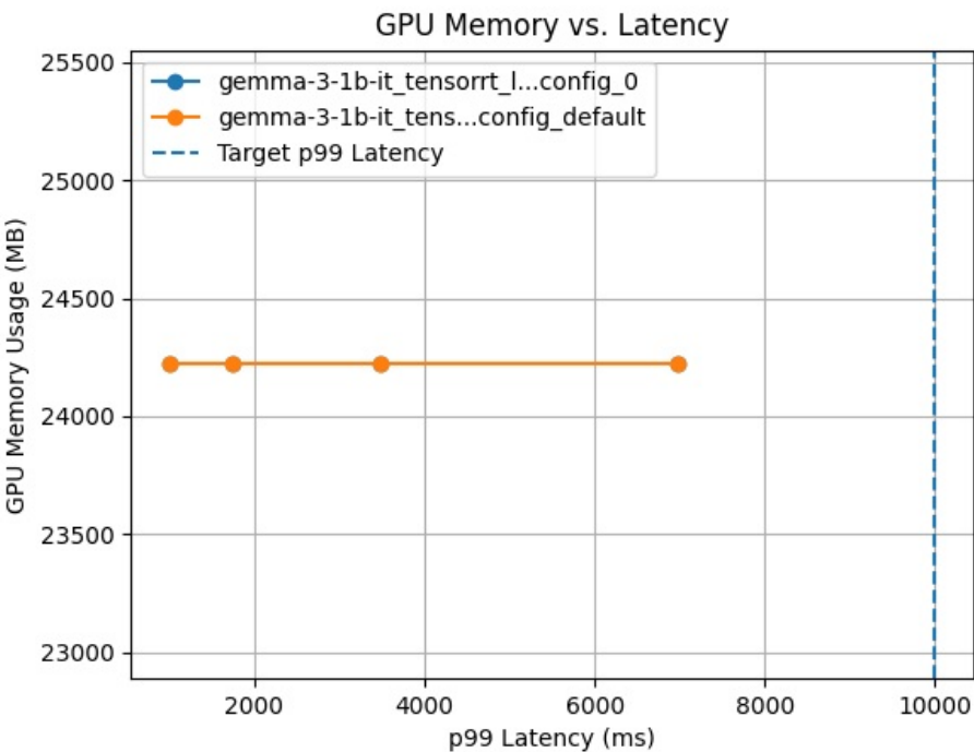
GPU Memory vs. Latency curves for 2 best configurations.
