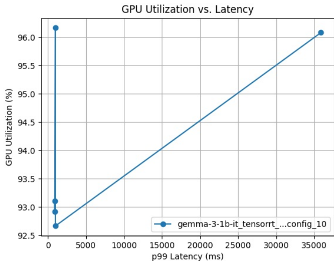
GPU Utilization vs. Latency curves for config gemma-3-1b-it_tensorrt_llm_bls_config_10
