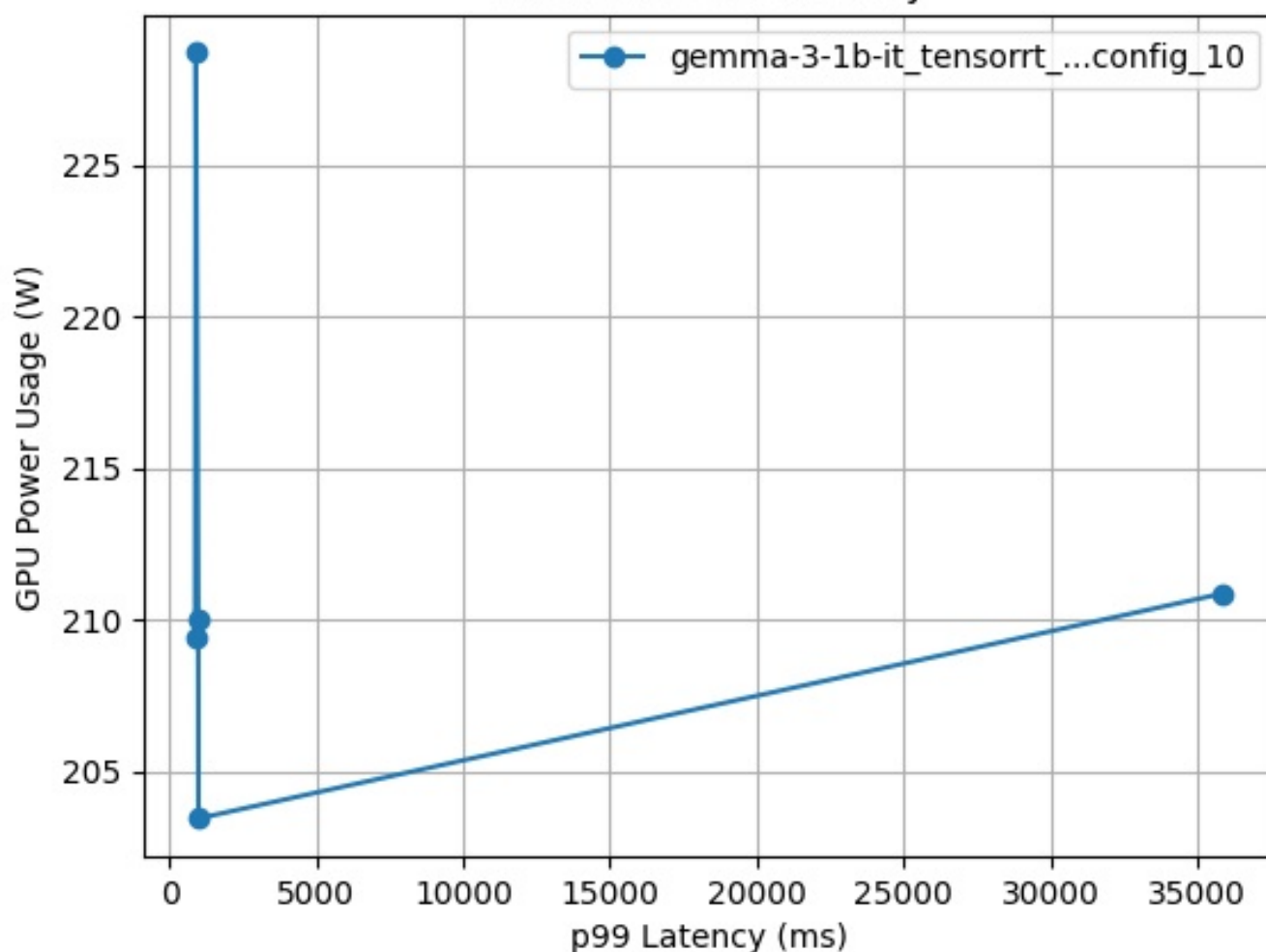
GPU Power vs. Latency curves for config gemma-3-1b-it_tensorrt_llm_bls_config_10
