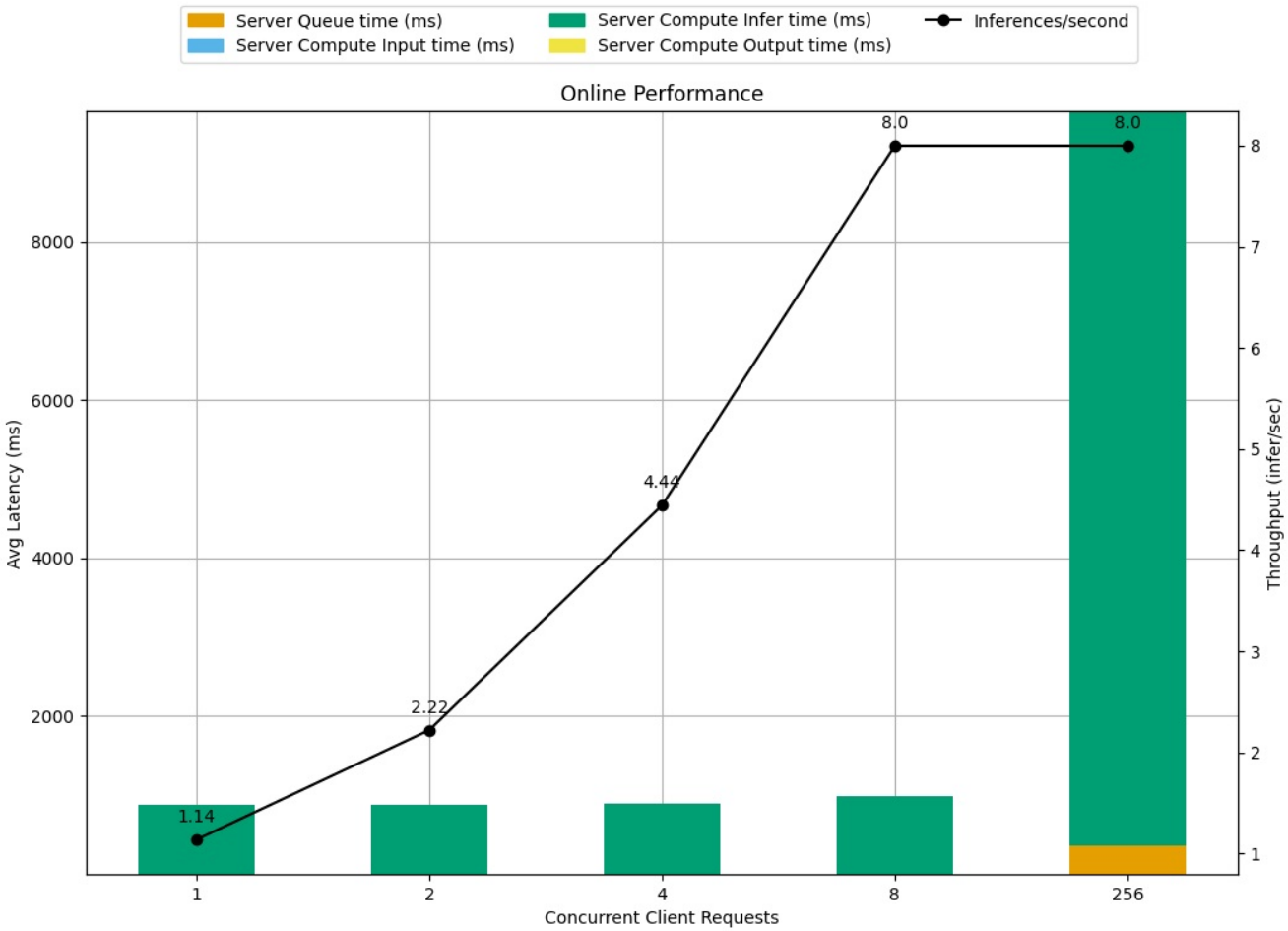
Latency Breakdown for Online Performance of gemma-3-1b-it_tensorrt_llm_bls_config_11
