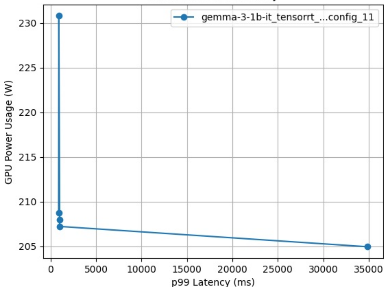
GPU Power vs. Latency curves for config gemma-3-1b-it_tensorrt_llm_bls_config_11
