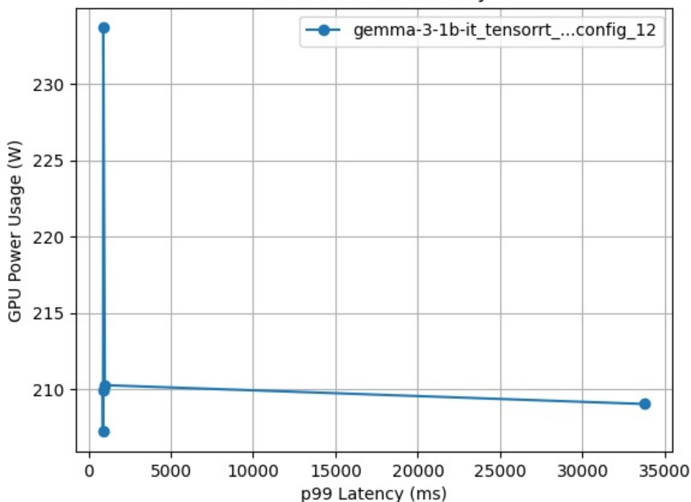
GPU Power vs. Latency curves for config gemma-3-1b-it_tensorrt_llm_bls_config_12
