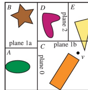
Axis Aligned Binary Space Partition Tree
