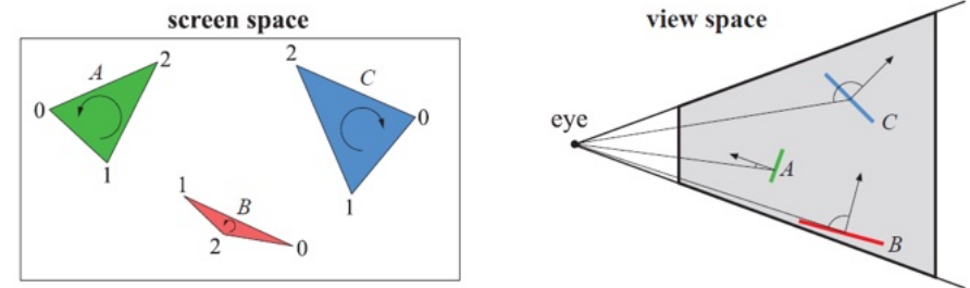
Backface culling
