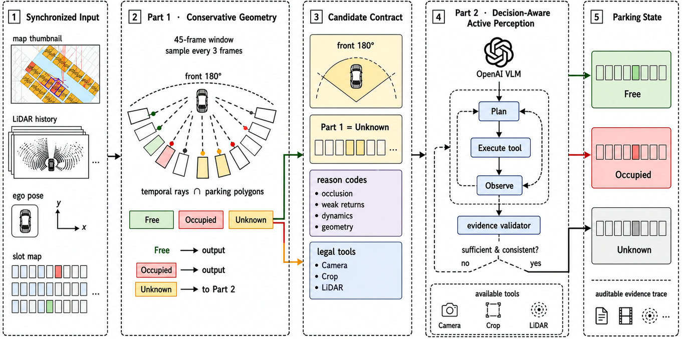
Fig. 1. DASP-Park system architecture. Causal map-aligned geometry separates terminal Free/Occupied evidence from unresolved Unknown cases. Only forward unresolved slots enter the camera-feasibility gate and the active-perception agent; an independent evidence validator controls final commitment.
