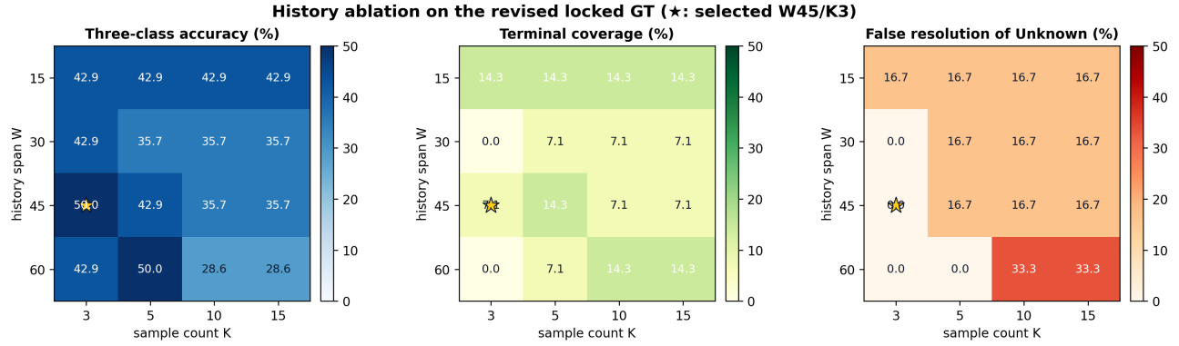
Fig. 4. Temporal-history ablation over all 16 ( W, K ) settings. The three heatmaps report overall three-class accuracy, terminal coverage, and false resolution of human-Unknown bays. The star marks the selected safety-first operating point W=45, K=3 .
