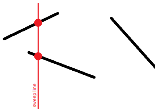
Figure 24.1: sweep line and line segment intersection
