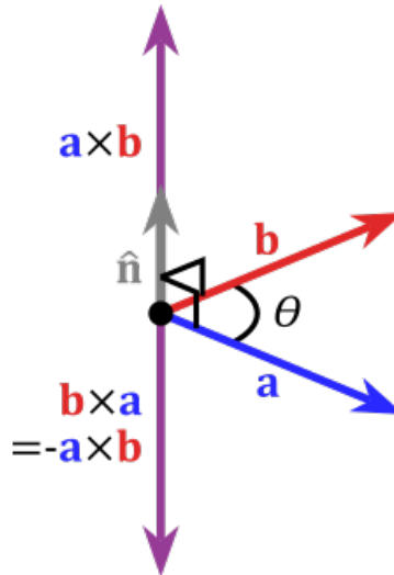
Figure 21.3: cross product
