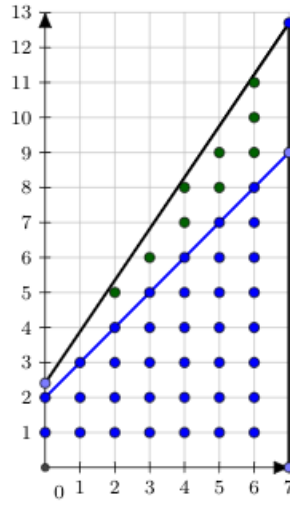
Figure 22.1: Subtracting floored linear function
