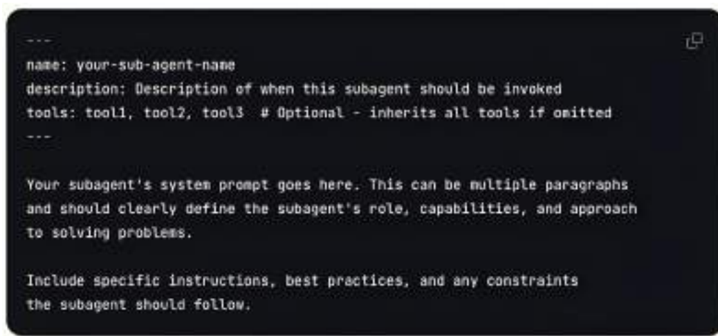
Figure 7.1 – Subagent file structure
