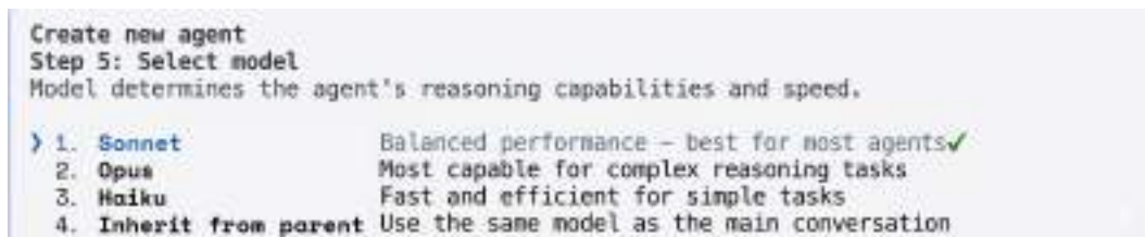
Figure 7.5 – Choosing the model and reviewing the subagent configuration summary
