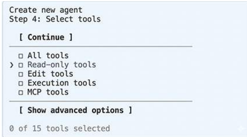
Figure 7.4 – List of tools for the subagent during setup
