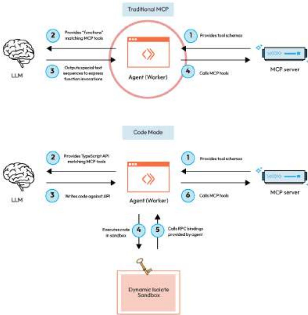
Figure 4.41 – Traditional MCP vs Code Mode execution flow
