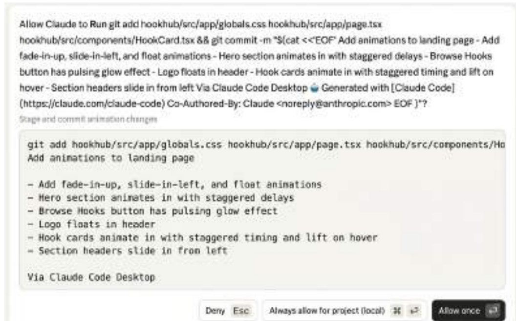
Figure 10.22 – Claude Code preparing a commit for the animation feature changes
