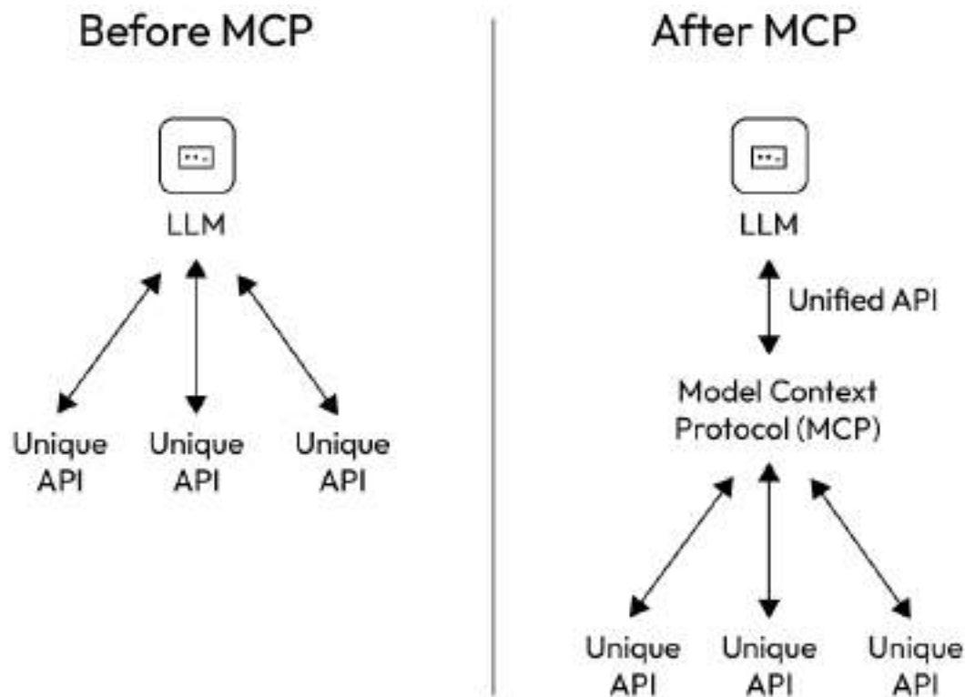
Figure 4.33 – MCP abstraction layer between LLMs and external APIs
