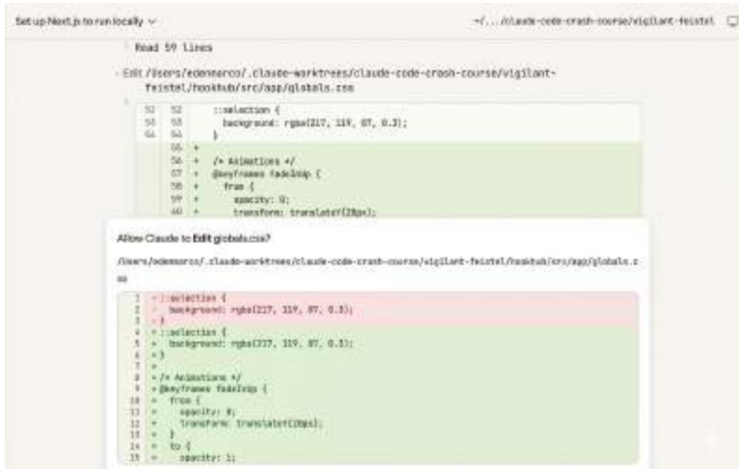
Figure 10.13 – Reviewing and approving local code changes generated by Claude Code
