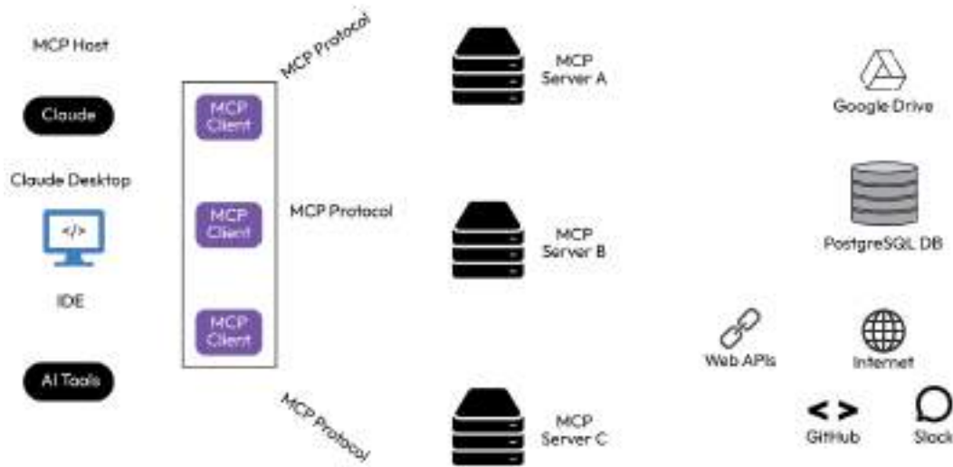
Figure 4.9 – MCP client inside the host managing communication with MCP servers
