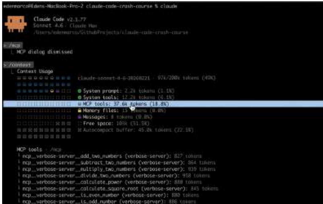
Figure 4.28 – MCP tools consuming a large portion of the context window
