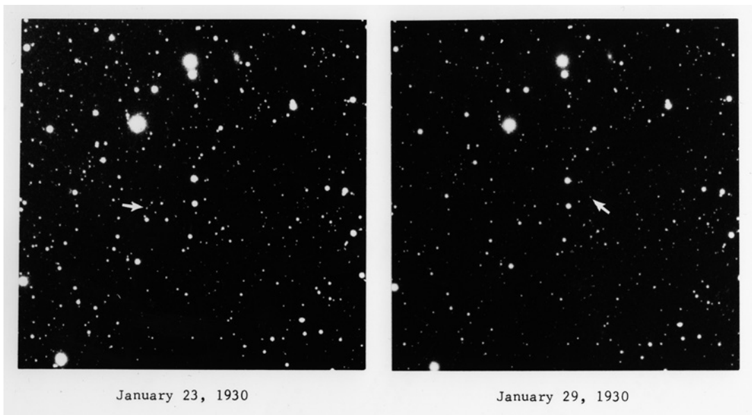
Figure 5-1: Discovery plates for Pluto, indicated by the arrow
