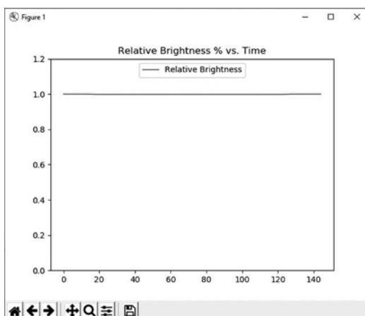
Figure 8-7: Light curve from Figure 8-6 with rescaled y-axis
