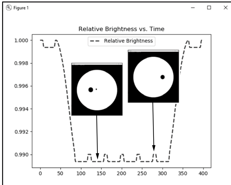
Figure A-1: Light curve for planet and moon where moon passes behind planet
