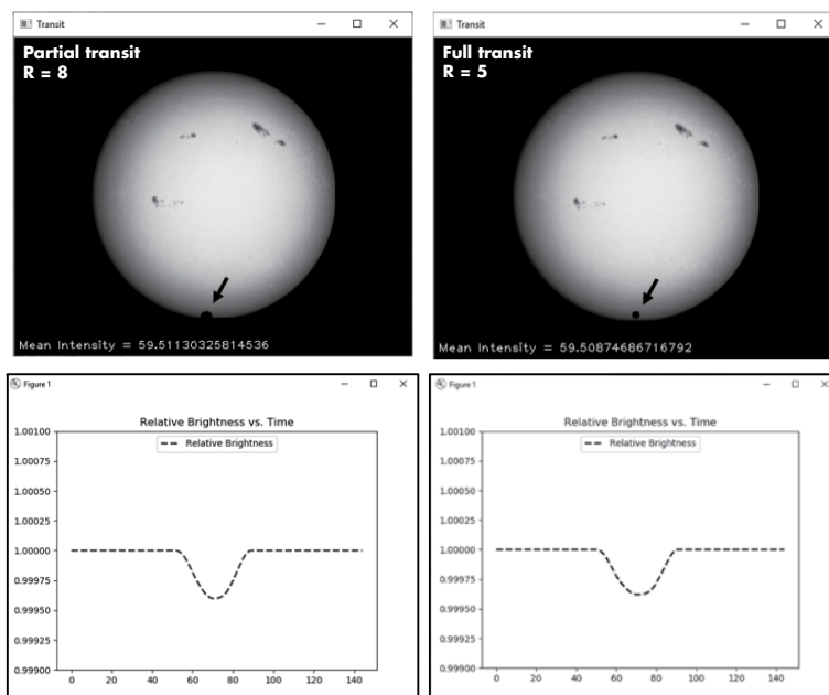
Figure 8-25: Partial transit of planet with a radius of 8 pixels versus full transit of planet with a radius of 5 pixels
