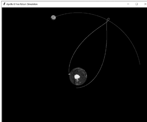
Figure 6-14: The simulation run with the pen down and the CM at splashdown in the Pacific
