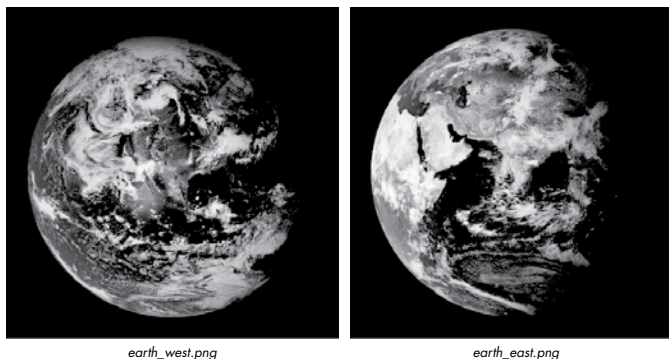
Figure 8-12: Images of the western and eastern hemispheres
