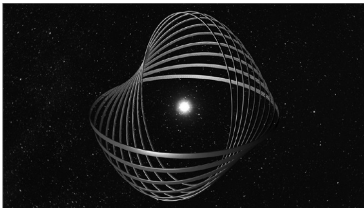
Figure 8-18: Pokrovsky shell system of rings around a star designed to intercept the star's radiation
