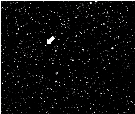
Figure 5-4: 1_bright_transient_left.png with an arrow indicating the transient
