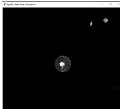
Figure 6-13: The simulation run with the pen up and the CSM approaching the moon
