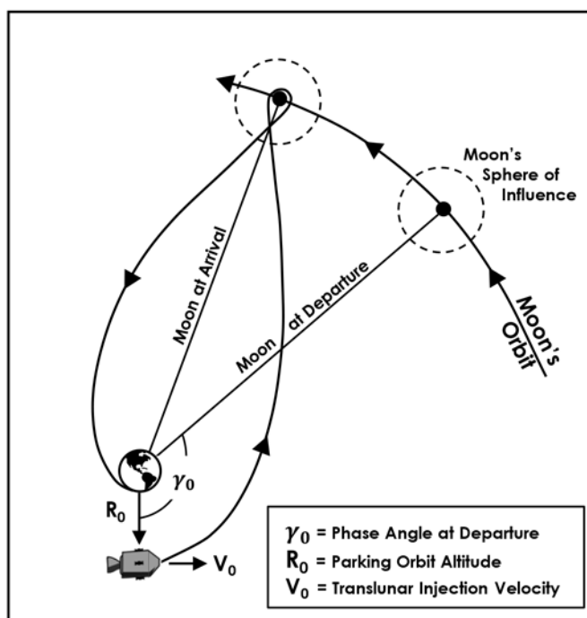
Figure 6-3: The free return trajectory (not to scale)
