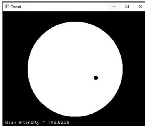
Figure 8-5: The exoplanet transiting the star
