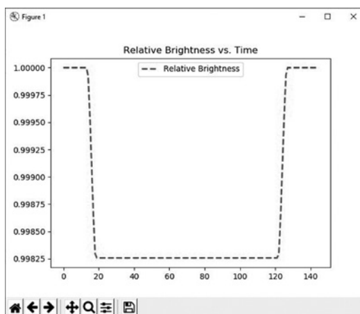
Figure 8-6: Example light curve plot from transit.py
