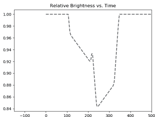
Figure 8-19: Light curve produced by practice_tabbys_star.py
