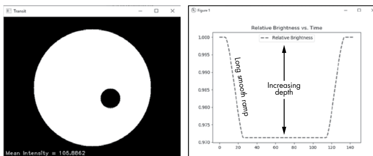
Figure 8-10: Light curve for EXO\_RADIUS = 28
