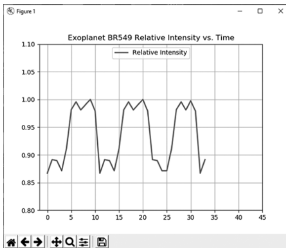
Figure 8-28: Composite light curve for 34 images of exoplanet BR549
