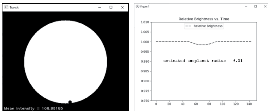
Figure 8-8: Light curve for an exoplanet with a radius of 7 that only partly crosses its star
