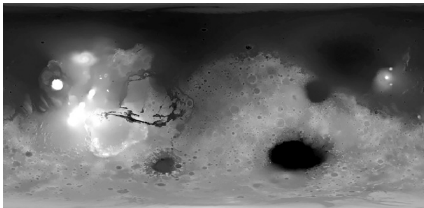
Figure 7-4: Mars MGS MOLA Digital Elevation Model 463m v2 (mola_1024x501.png)
