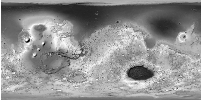
Figure 7-2: MOLA shaded relief map of Mars
