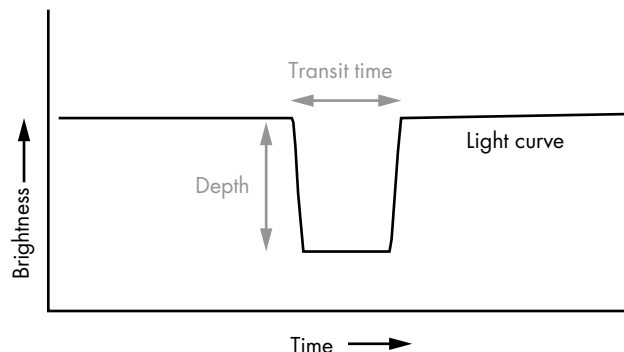
Figure 8-3: Depth represents the total change in brightness observed in a light curve.
