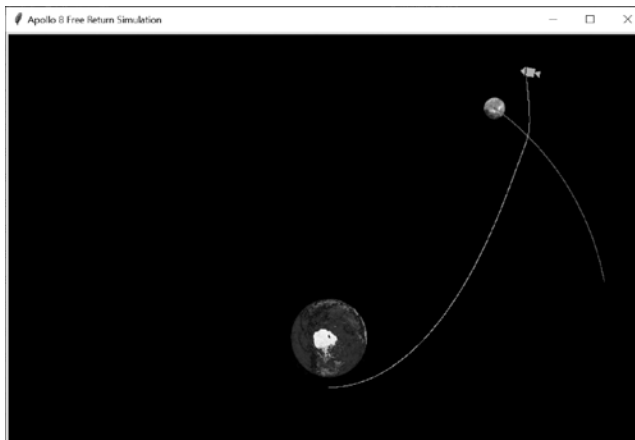
Figure 6-15: The gravitational slingshot maneuver achieved with Vo_X = 520
