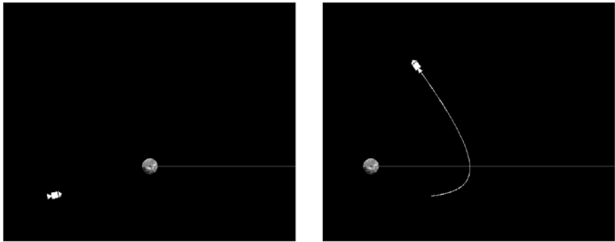
Figure 6-18: The moon approaches a stationary CSM (left) and then flings it to the stars (right).
