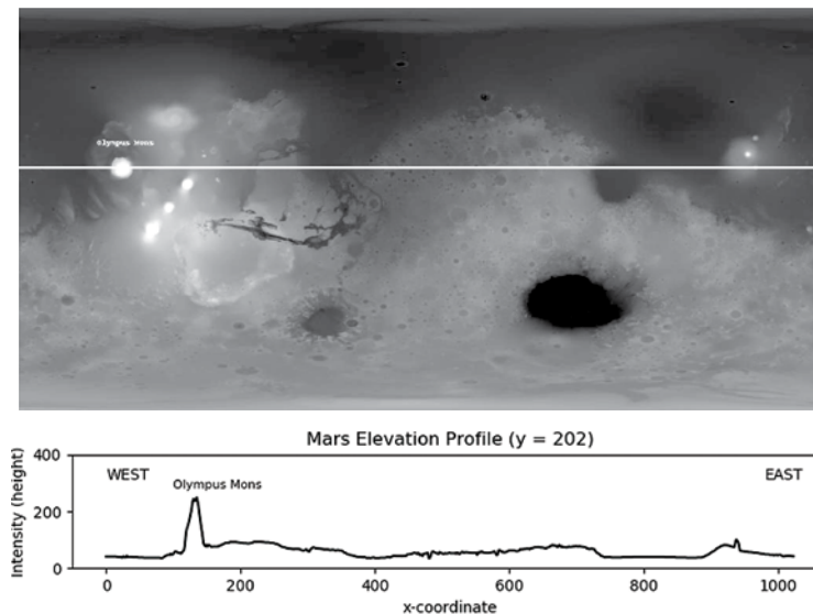
Figure 7-15: Vertically exaggerated west-east profile through Olympus Mons
