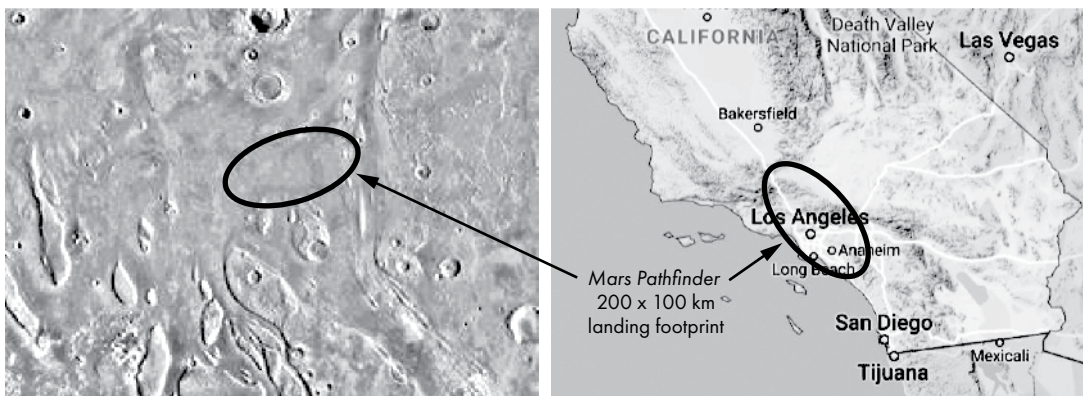
Figure 7-1: Scaled comparison of 1997 Mars Pathfinder landing site (left) with Southern California (right)
