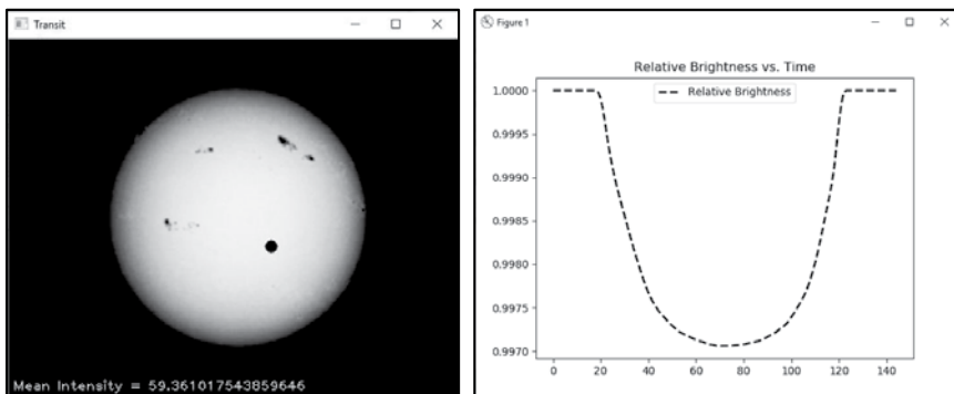
Figure 8-23: The effect of limb darkening on a light curve
