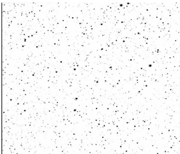
Figure 5-10: The negative image, 6_bright_transient_neg_left_registered.png
