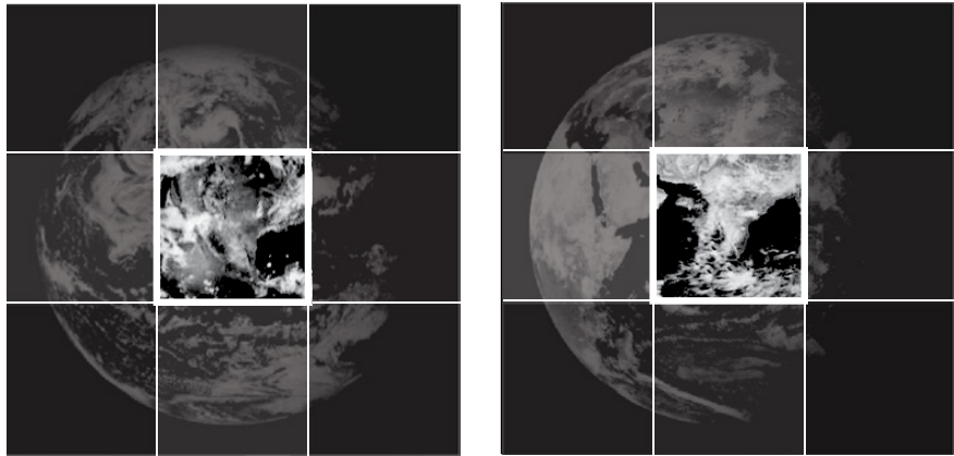
Figure 8-13: The earth_west.png and earth_east.png images overlaid with a 9-pixel grid
