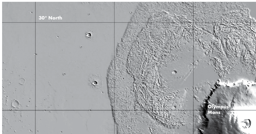
Figure 7-14: The very smooth terrain west of the Olympus Mons lava fields
