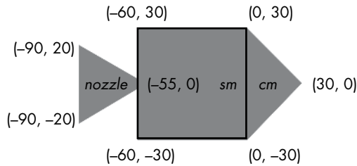
Figure 6-12: CSM compound shape with coordinates for nozzle, service module, and command module
