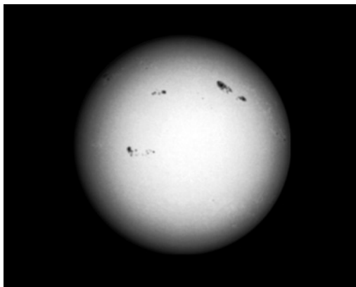
Figure 8-22: Limb darkening and sunspots on the sun
