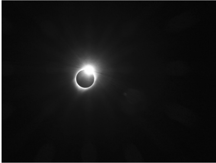
Figure 8-4: Diamond ring effect at the end of totality, 2017 solar eclipse
