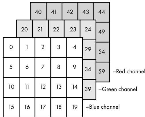
Figure 1-4: Visual representation of a three-channel color image array
