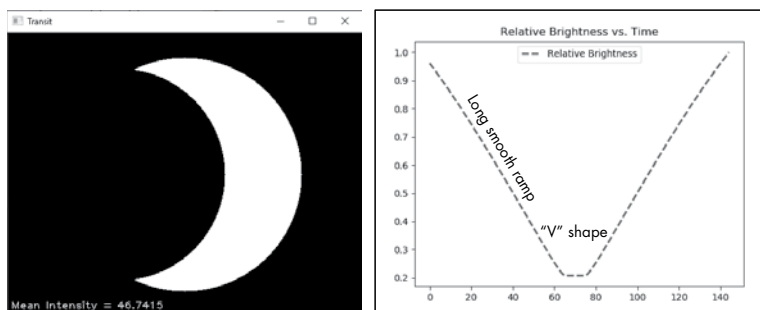
Figure 8-11: Light curve for EXO\_RADIUS = 145
