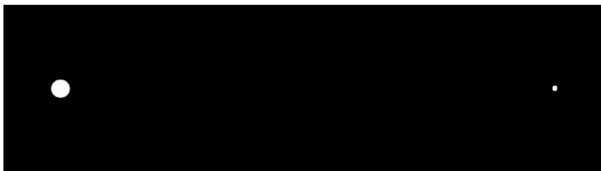
Figure 6-10: Earth and moon system at closest approach, or perigee, shown to scale
