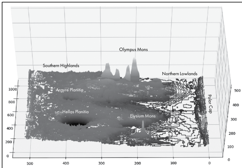
Figure 7-16: A 3D contour plot of Mars, looking toward the west
