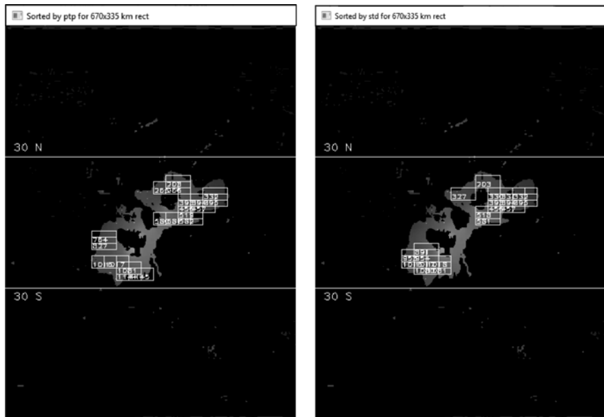
Figure 7-18: Filtered MOLA map over the Tharsis Montes region, with ptp (left) and std (right) rectangles
