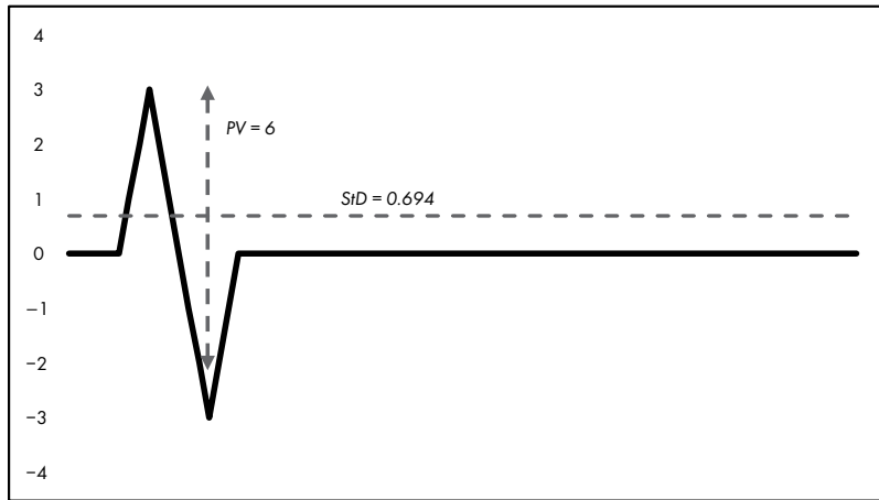
Figure 7-3: A surface profile (black line) with standard deviation (StD) and peak-to-valley (PV) statistics
