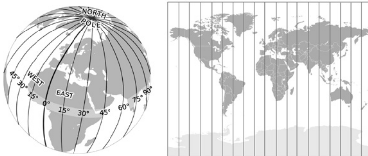
Figure 7-7: Forcing lines of longitude to be parallel distorts the size of features near the poles.
