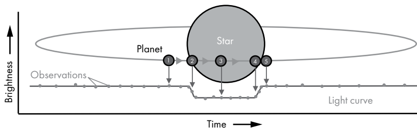
Figure 8-2: The transit photometry technique for detecting exoplanets
