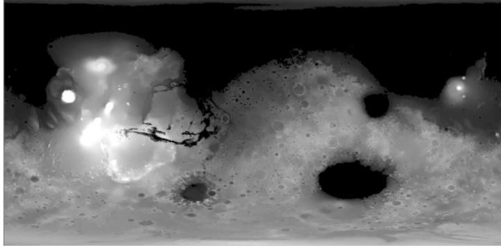
Figure 7-5: MOLA map with pixel values \leq 55 colored black to represent ancient Martian oceans
