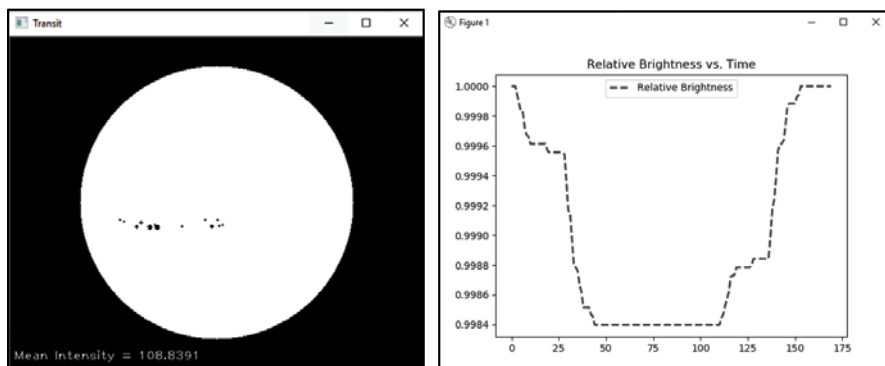
Figure 8-21: Irregular, asymmetrical light curve produced by a randomly generated asteroid field
