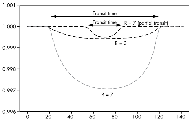
Figure 8-24: Limb-darkened light curves for full and partial transits ( R = exoplanet radius)
