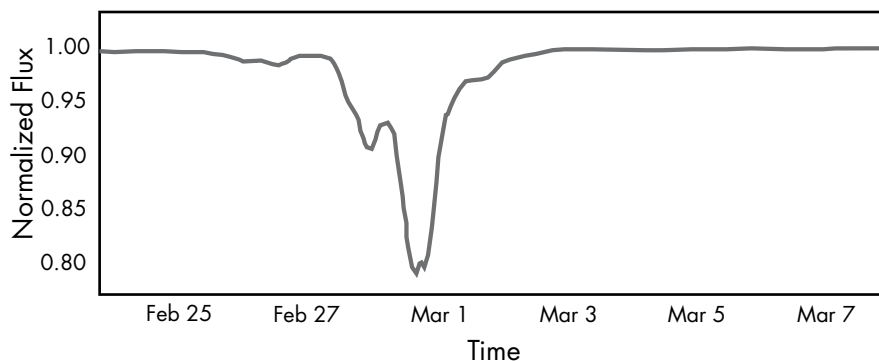
Figure 8-17: Light curve for Tabby’s Star, measured by the Kepler Space Observatory
