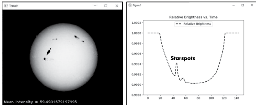
Figure 8-26: An exoplanet (arrow, left image) passing over a starspot produces a bump in the light curve.
