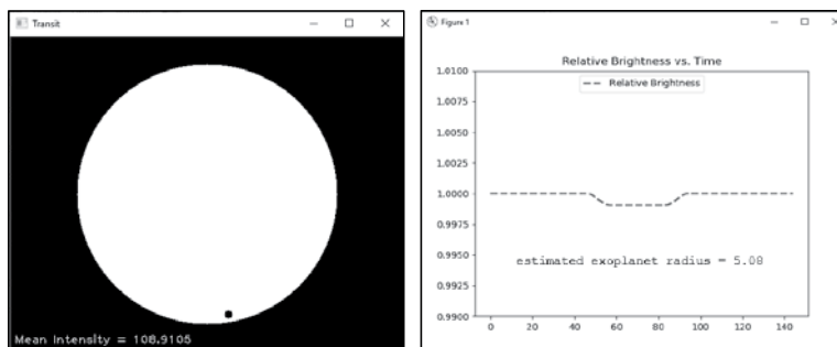
Figure 8-9: Light curve for an exoplanet with a radius of 5 that fully crosses its star
