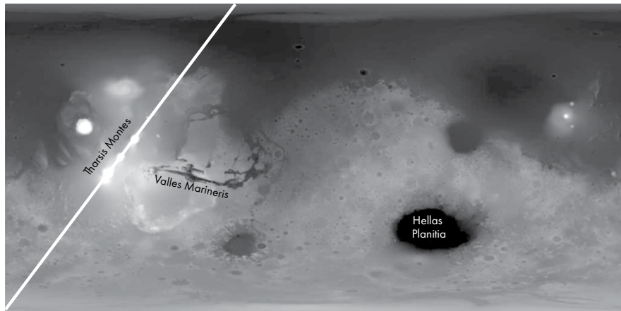
Figure 7-19: Diagonal profile through the three volcanoes on Tharsis Montes
