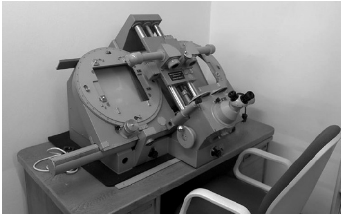
Figure 5-2: A blink comparator
