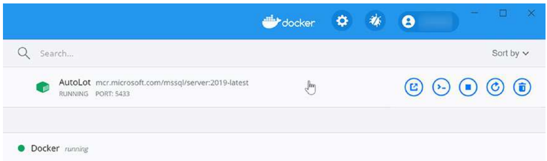
Figure 20-2. Docker Dashboard
