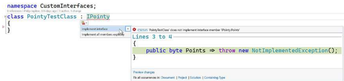
Figure 8-5. Implementing interfaces automatically using Visual Studio
