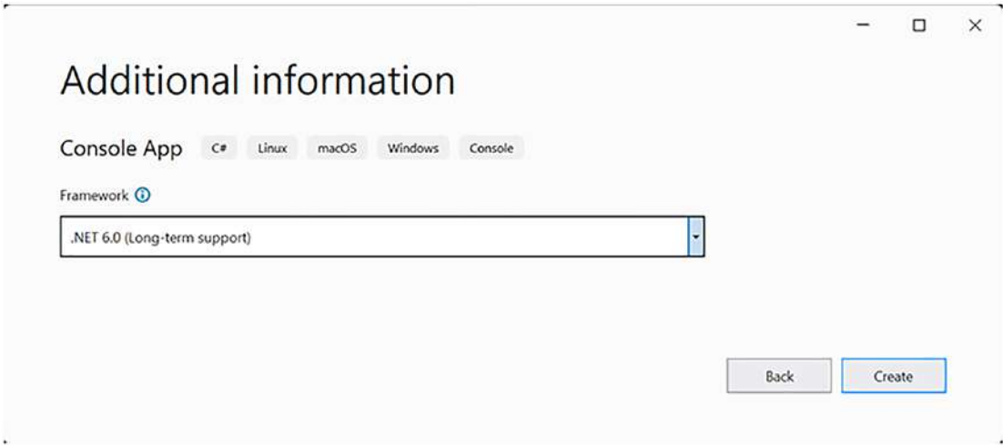
Figure 2-5. Chosing the .NET Version
