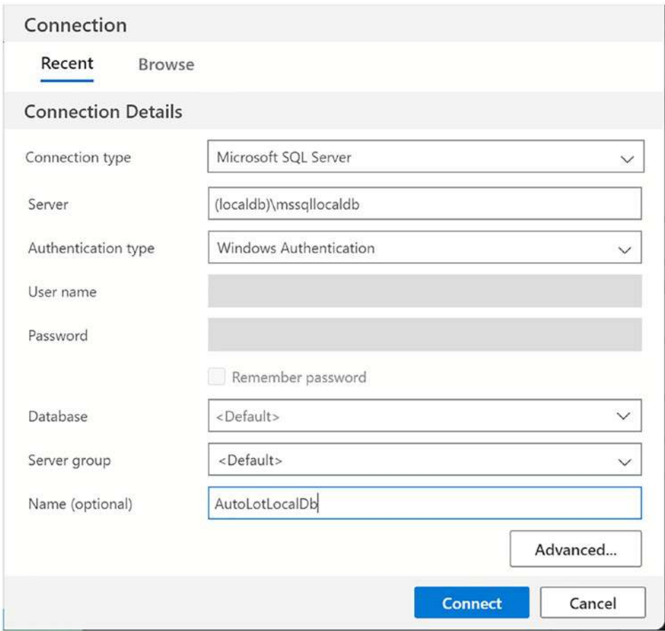
Figure 20-5. Setting the connection options for SQL Server LocalDb
