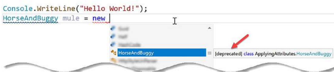
Figure 17-1. Attributes in action in Visual Studio
