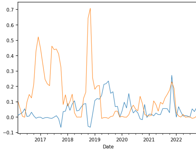
Figure 5.9: Rolling marginal contribution to risk for the two Fama-French factors
