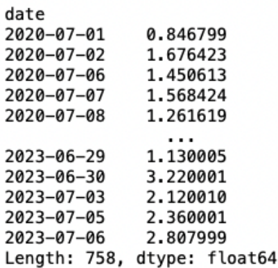
Figure 2.30: Series with the range of AAPL stock
