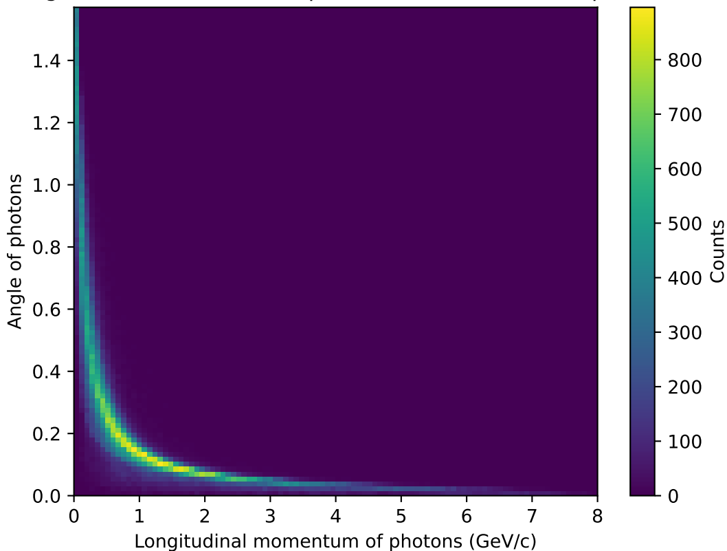
Angles and momentum of photons, 300 MeV/c 2 in prima
