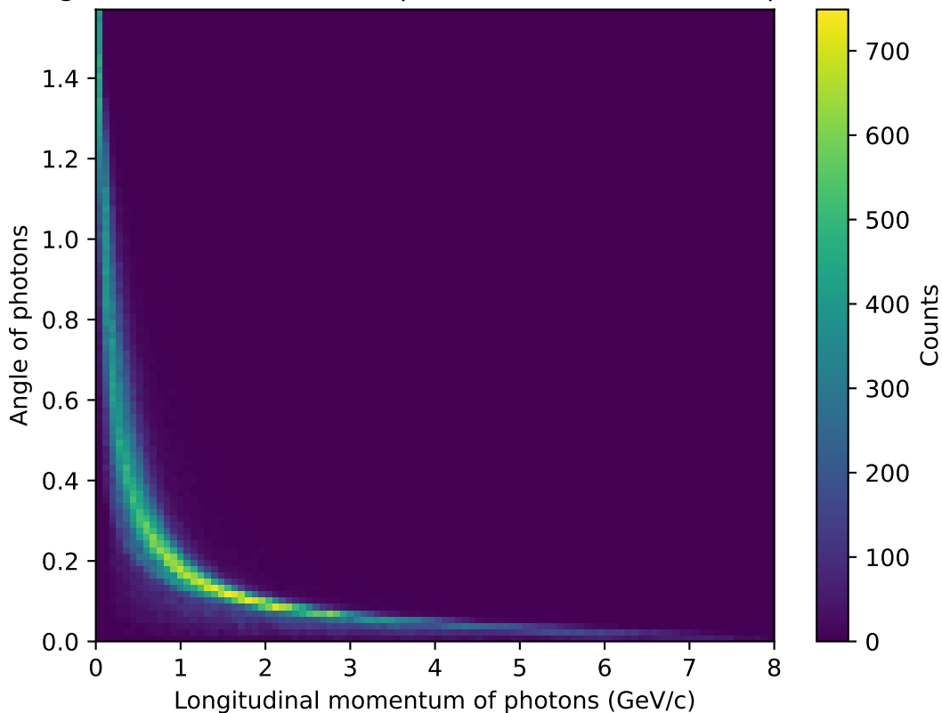
Angles and momentum of photons, 400 MeV/c 2 in prima
