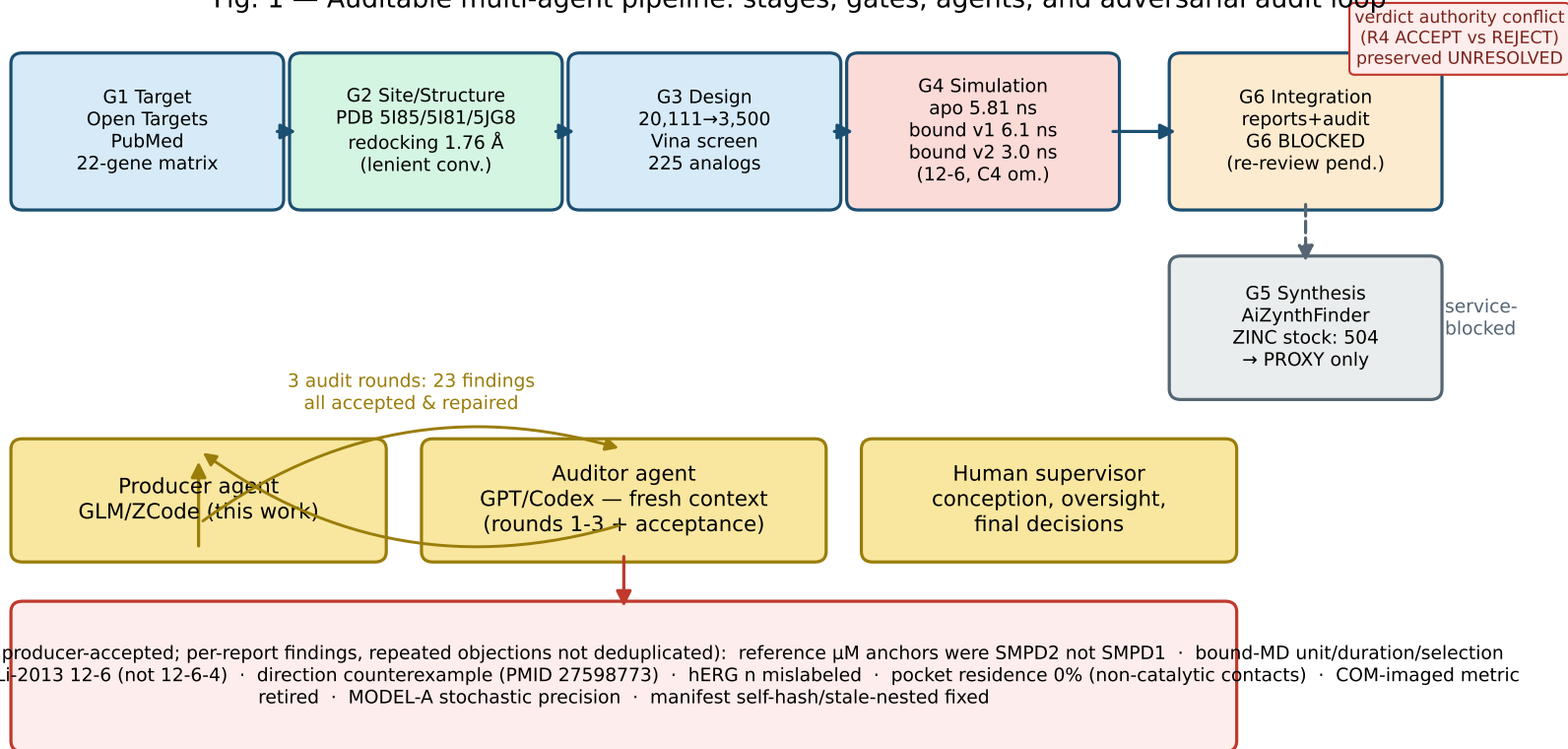
Fig. 1 — Auditable multi-agent pipeline: stages, gates, agents, and adversarial audit loop
