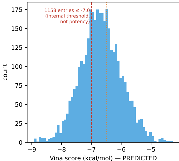
B score distribution (best -8.92 CHEMBL54786)
