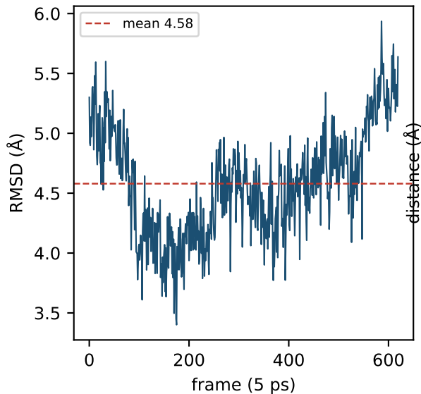
A ligand RMSD in protein frame
