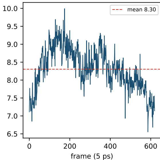
B ligand COM dist to crystal centroid
