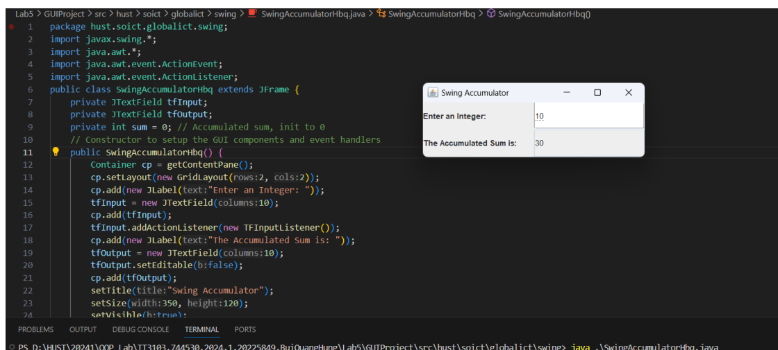
Figure 1.3 Source code of SwingAccumulator
