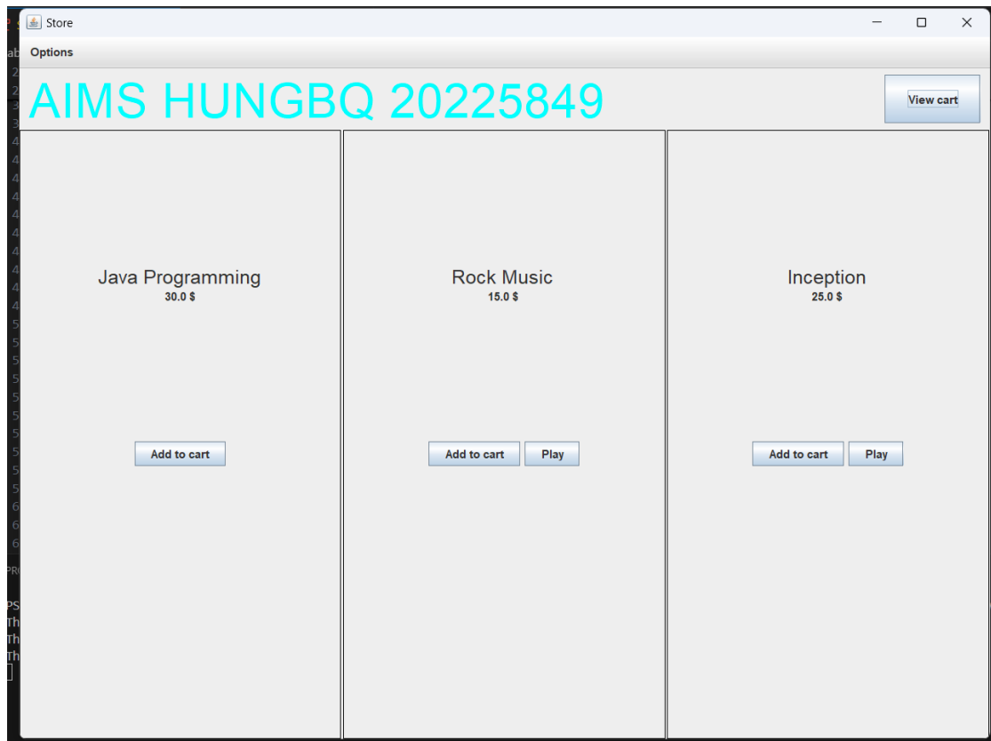
Figure 3.7 StoreScreen
