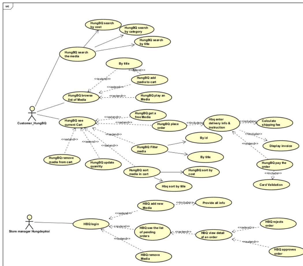
Figure 9.1 Usecase Diagram
