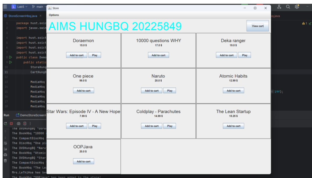
Figure 8.3 Store after add book
