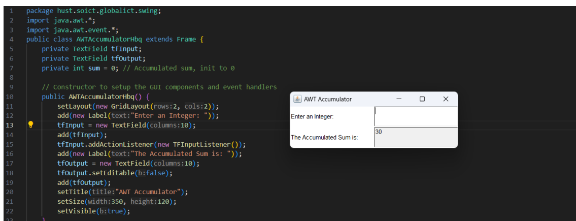
Figure 1.2 Demo of AWTAccumulator
