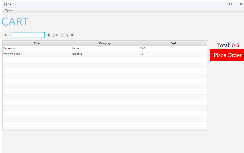
Figure 5.9 CartScreen Demo
