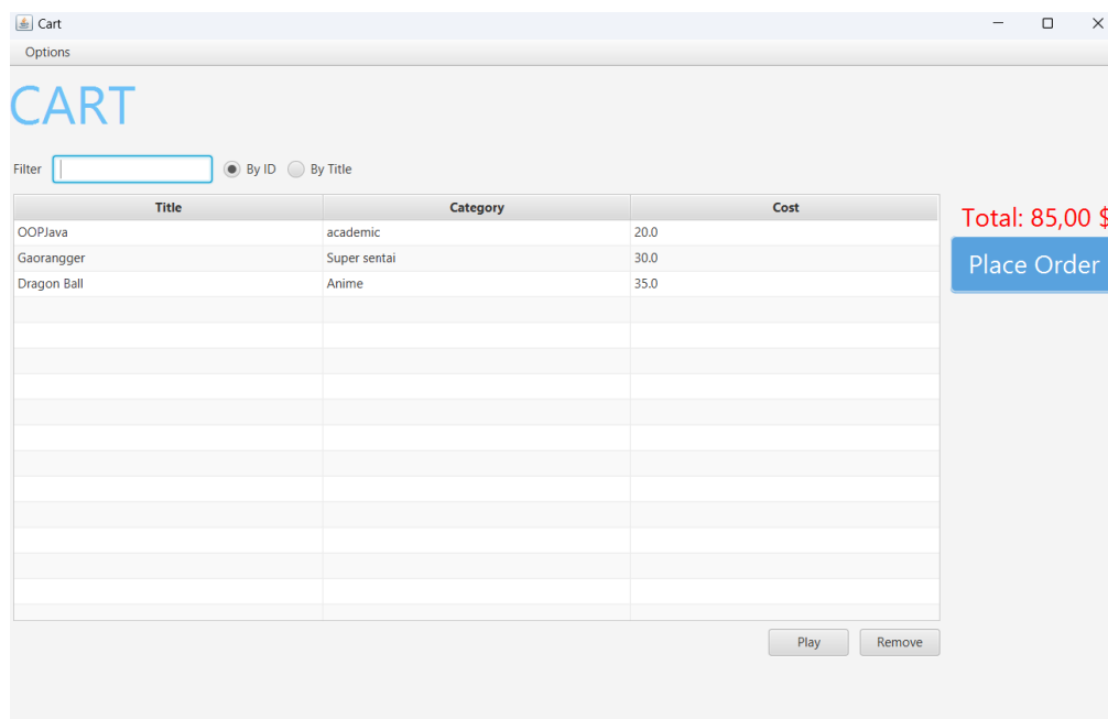
Figure 8.8 Cart
