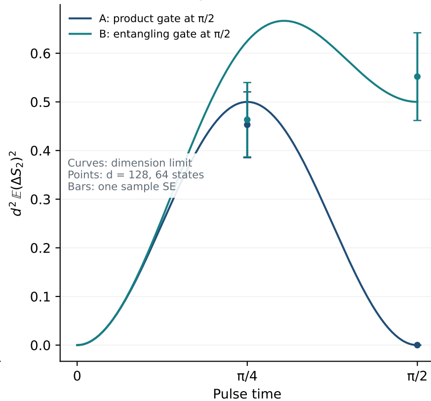
Matched energies: recurrence contrast
