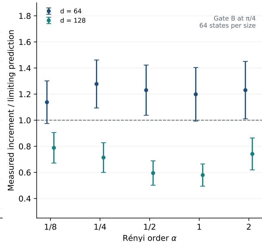
Finite-size deviations retained
