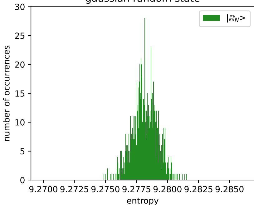
gaussian random state
