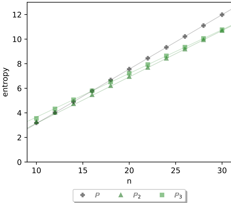
k-almost Prime states
