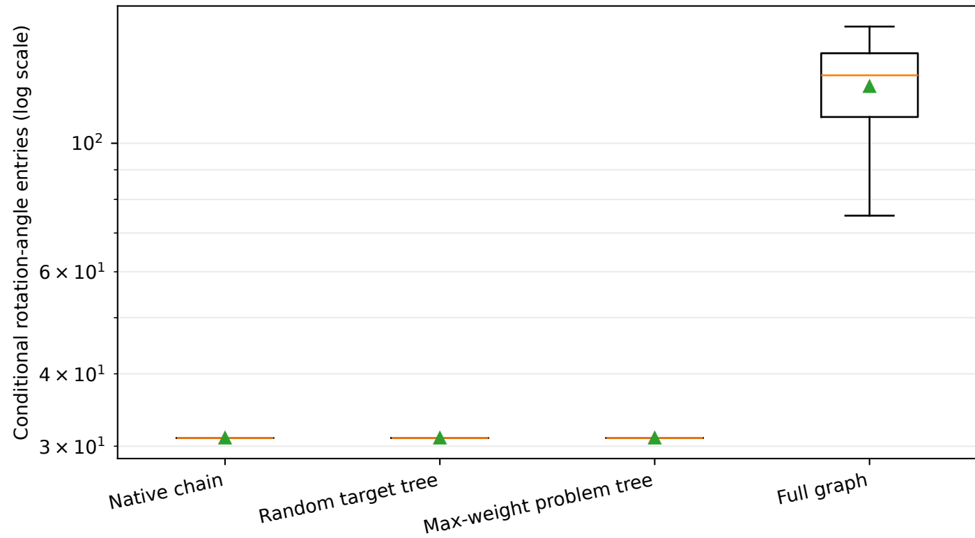
Exact q-sample representation cost
