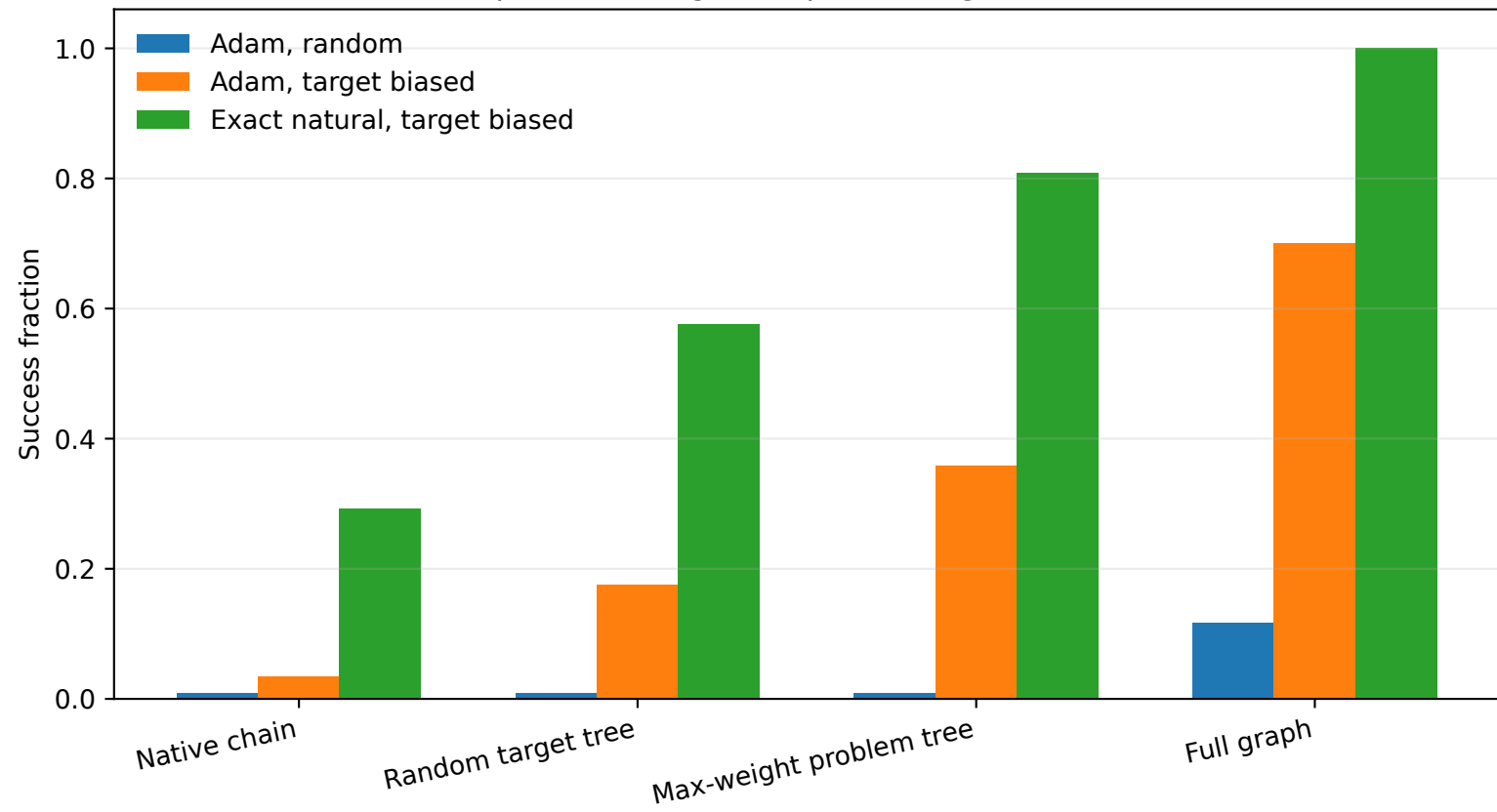
Independent weighted sparse-Ising confirmation
