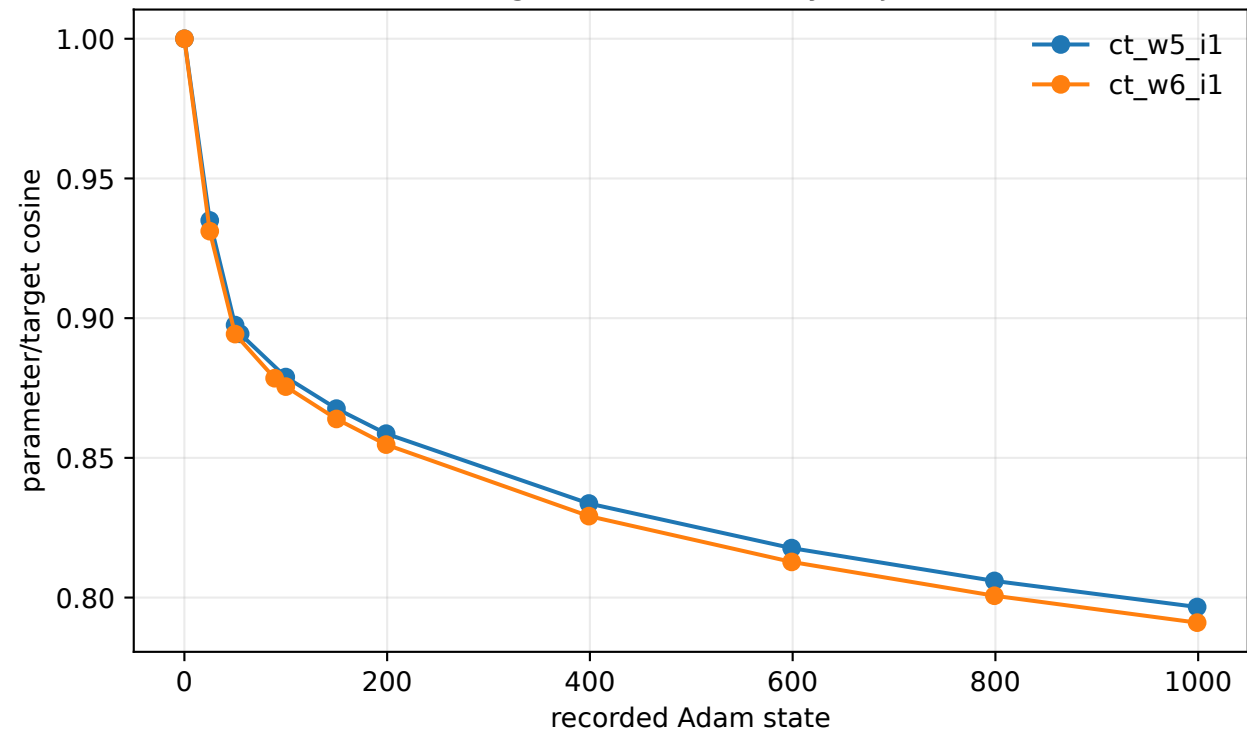
Exact-target Adam boundary trajectories
