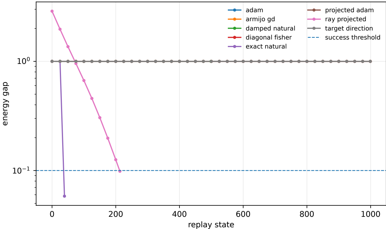
ct w5 i1: replay from Adam state 999
