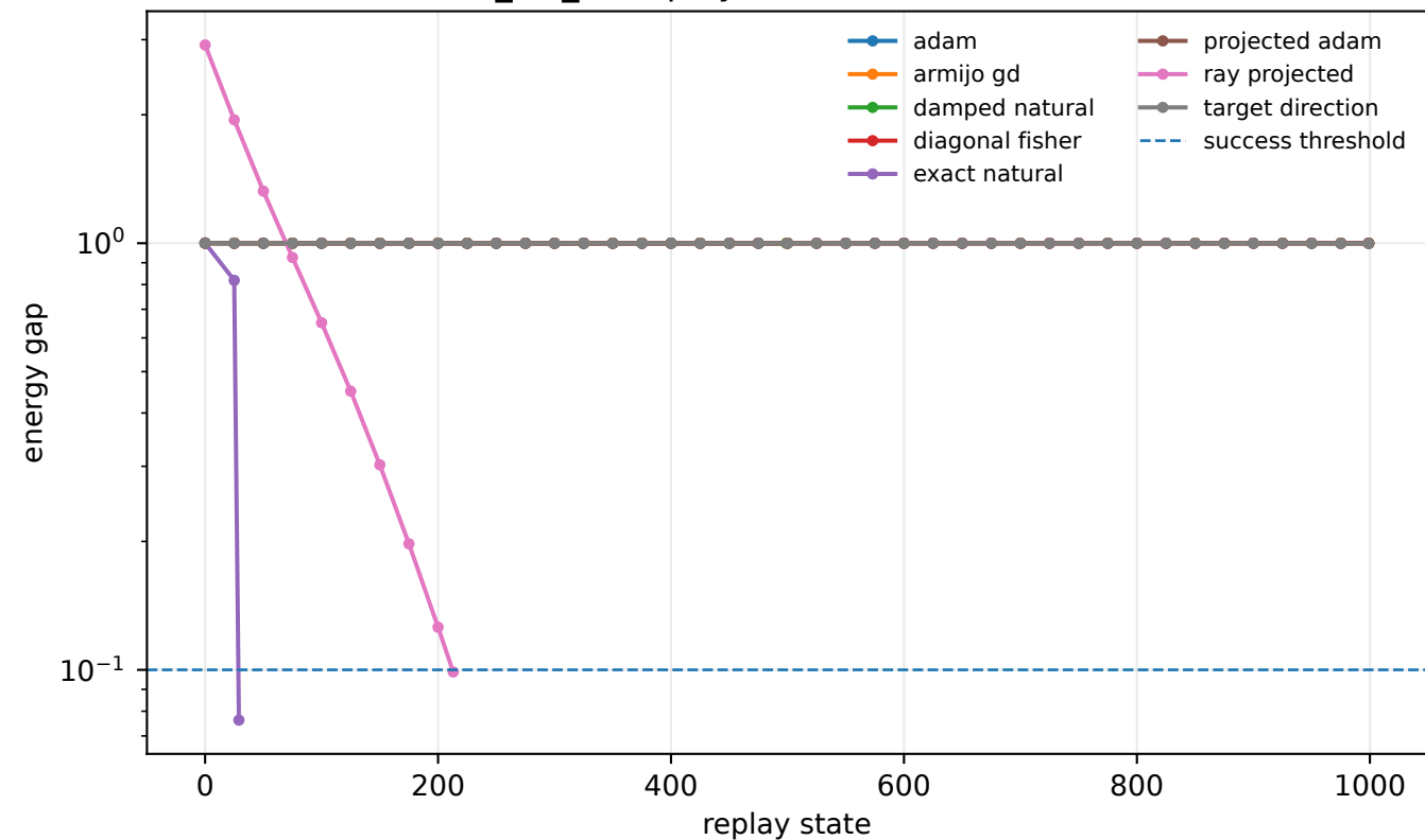
ct_w6_i1: replay from Adam state 999
