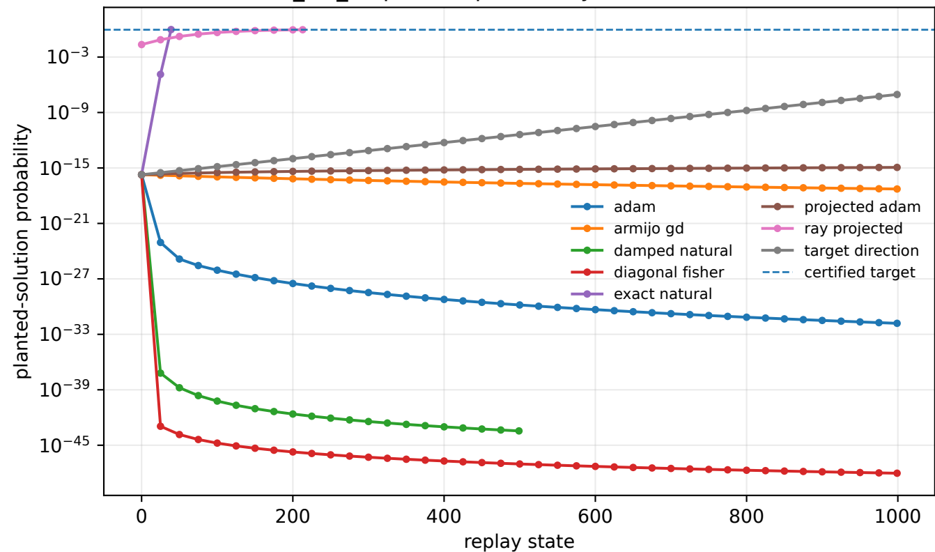
ct_w5_i1: planted probability from state 999
