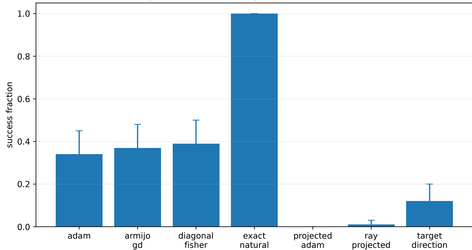
Optimizer success: target biased initialization
