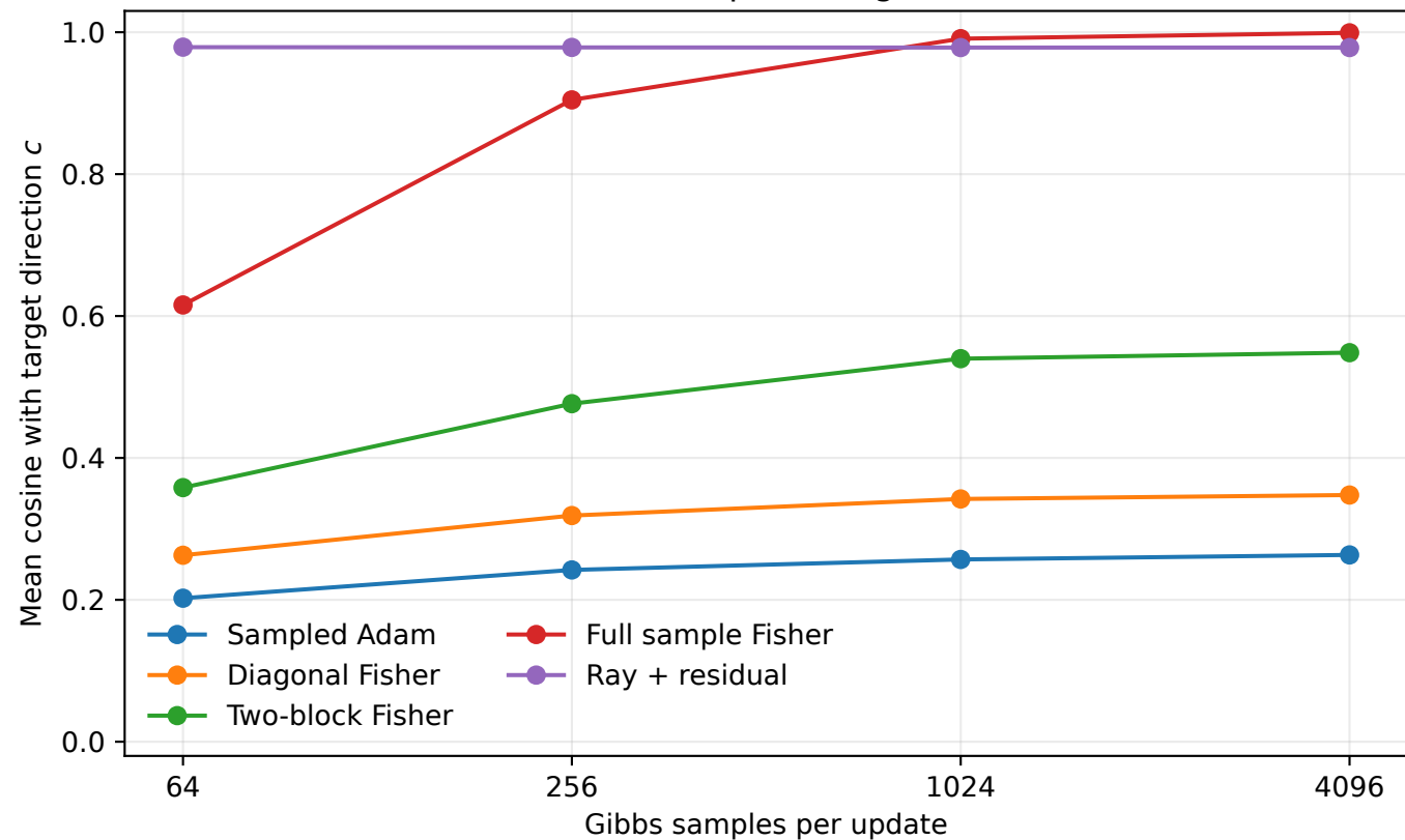
Estimated update alignment
