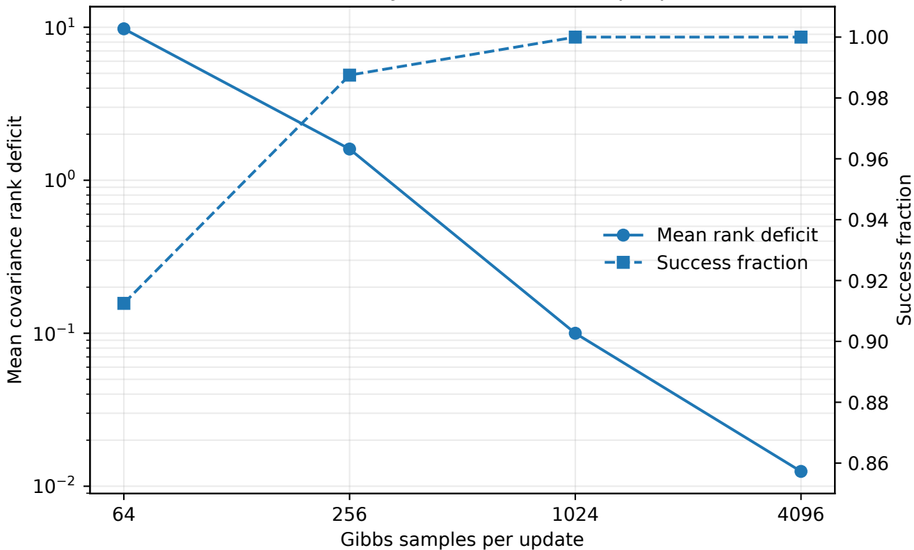
Full Fisher: rank recovery controls finite-sample performance
