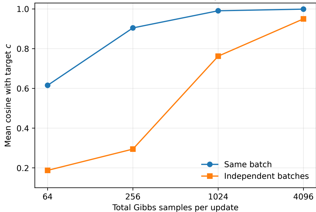
Direction recovery
