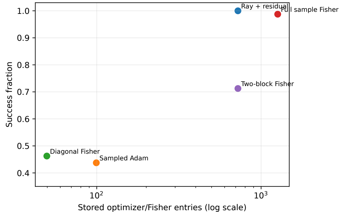
256 samples/update
