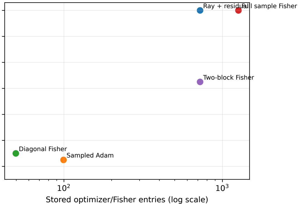
1024 samples/update
